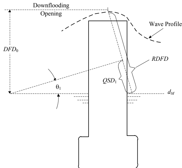
FIGURE 4 Downflooding Criterion
