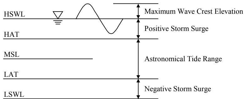
FIGURE 1 Definition of Water Levels
