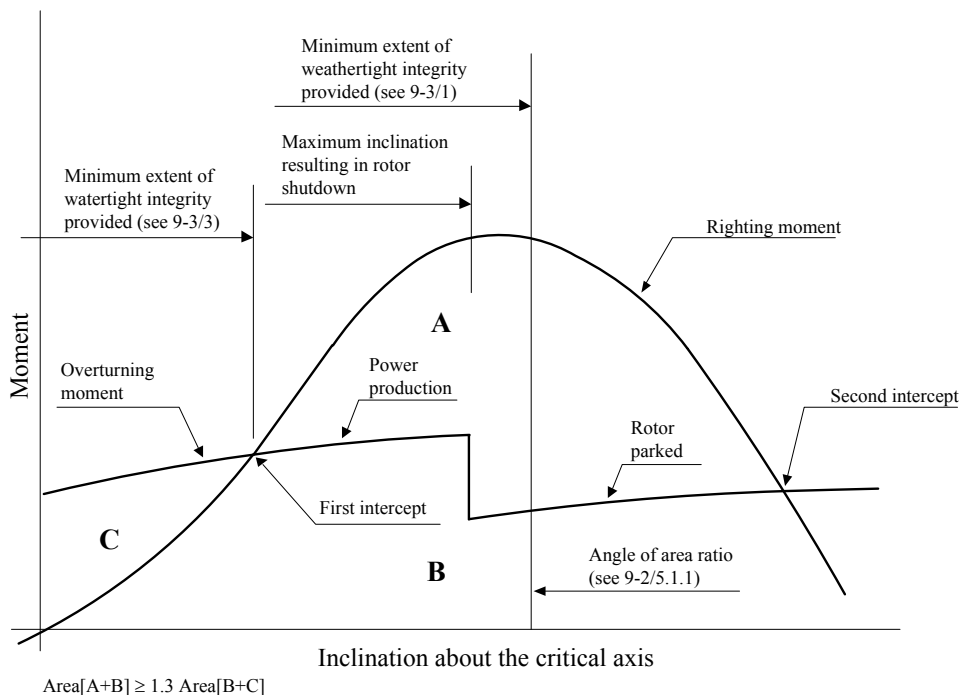
FIGURE 1 Intact Stability Curve for the RNA in Power Production
