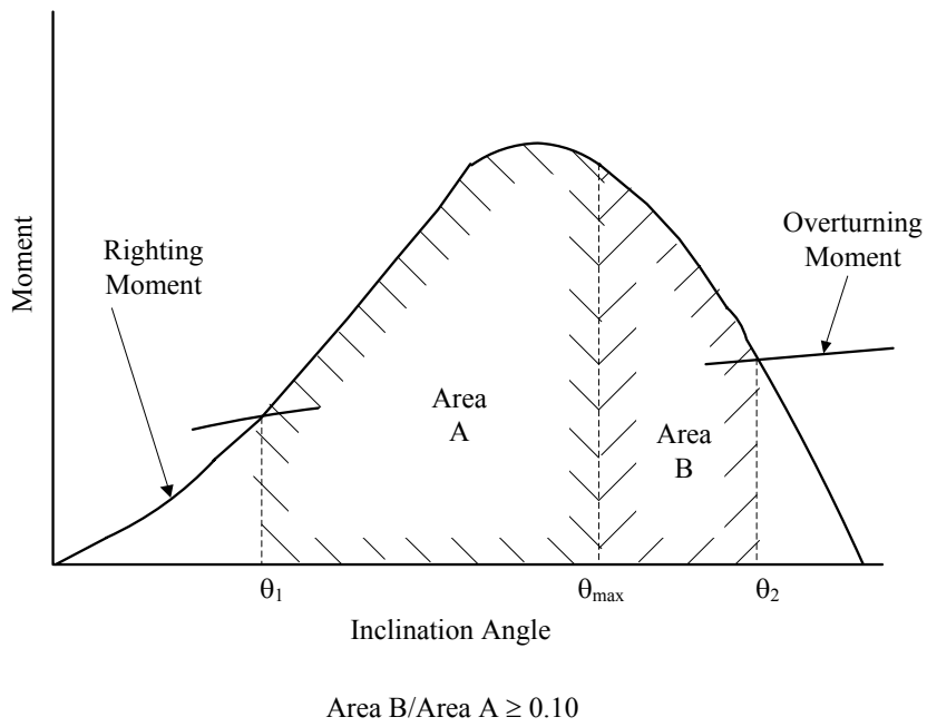
FIGURE 3 Capsize Criterion
