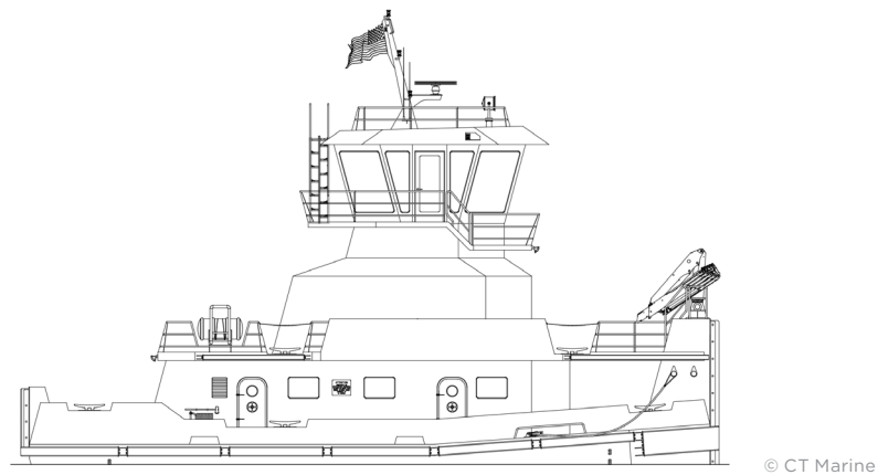
Figure A-5. Converted Electric Boat – Outboard Profile. 1220 BHP Zero-Emission Towboat.
