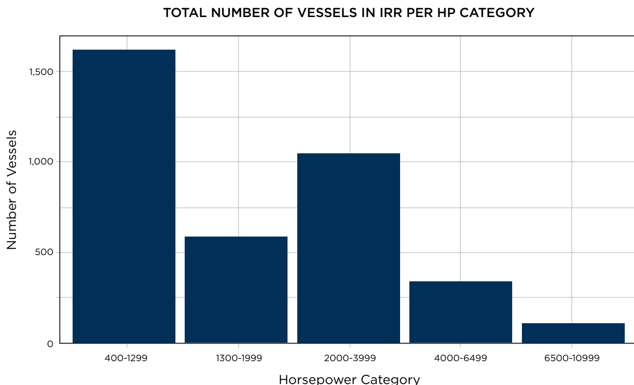
Figure 14. Industry fleet profile: Total number of vessels (as identified in the Inland River Record dataset) in relevant horsepower classes
