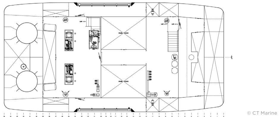
Figure A-2. Conventional Diesel Fuel Boat – Hold and Machinery Arrangement. 68' x 34' x 10' Twin Screw Z-Drive Towboat.
