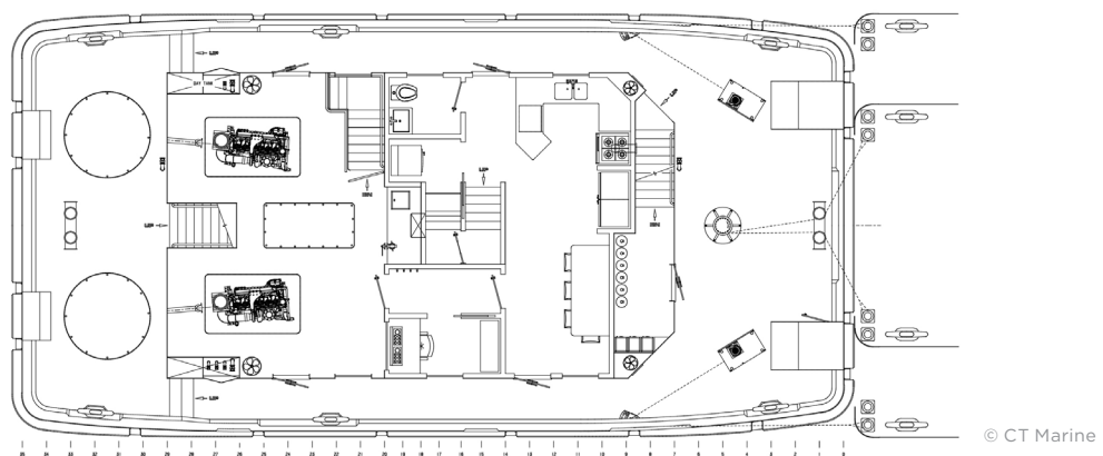
Figure A-3. Conventional Diesel Fuel Boat – Main Deck General Arrangement. 68' x 34' x 10' Twin Screw Z-Drive Towboat.
