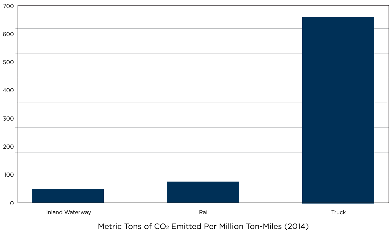
Figure 17. GHG intensity by mode. Source: Texas Transportation Institute (2017)
