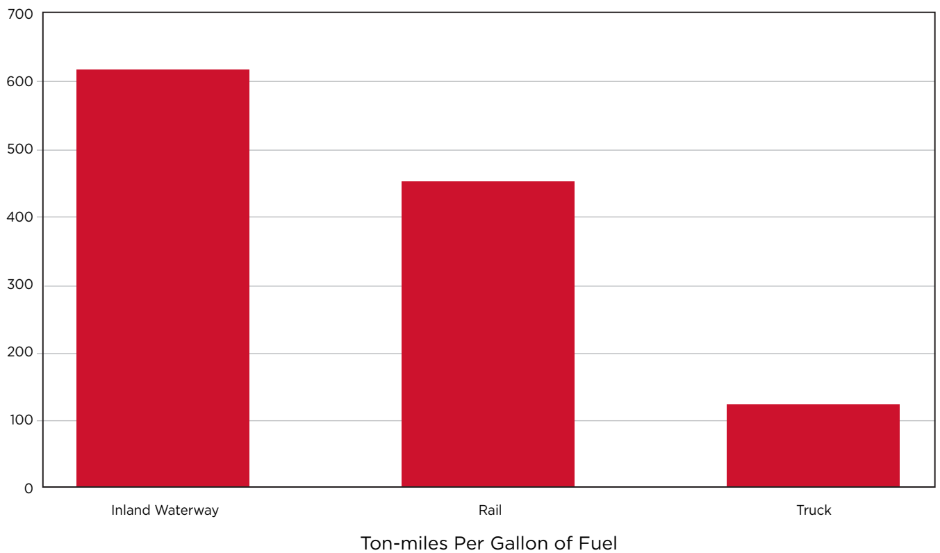
Figure 16. Fuel intensity by transportation mode. Source: Texas Transportation Institute (2017)
