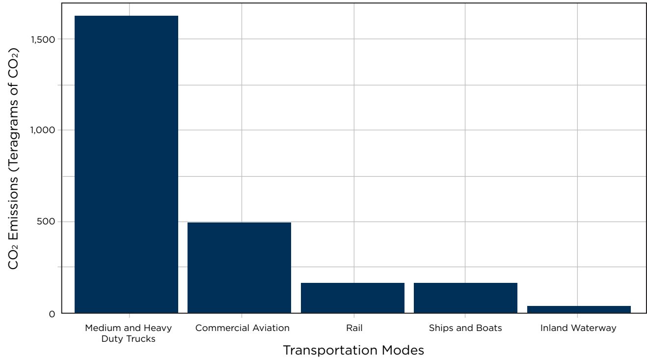
Figure 15. GHG emissions modal comparison. Commercial Aviation does not include passenger air traffic. Ships and Boats category may include some inland waterway. Data for inland waterways was calculated as part of this project; data for other modes was obtained from EPA’s annual GHG inventory.
