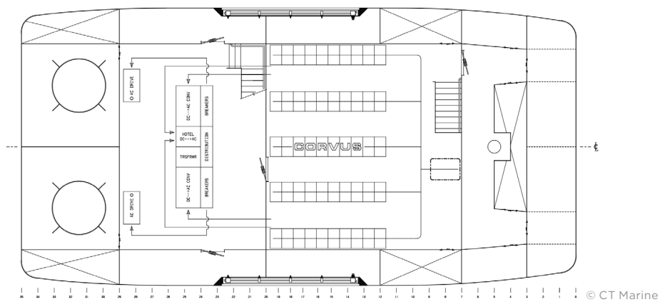
Figure A-4. Converted Electric Boat – Hold Plan. 1220 BHP Zero-Emission Towboat.
