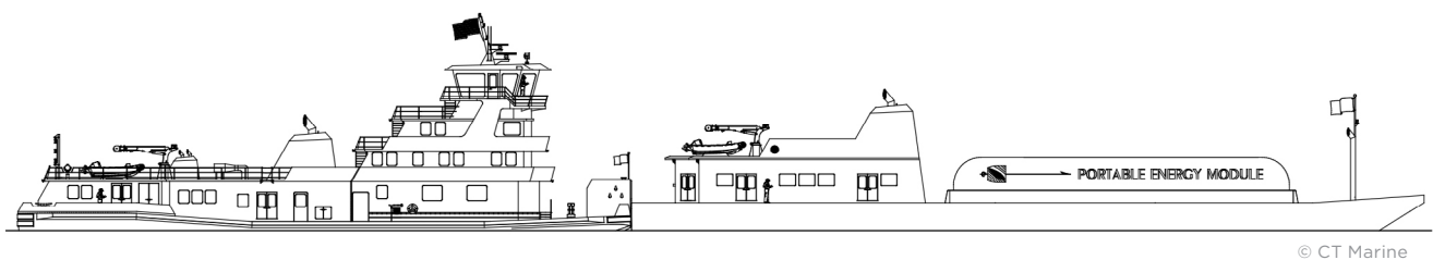
Figure 23. PEM Rendering. The PEM would be attached to the towboat along with the barge assembly.
