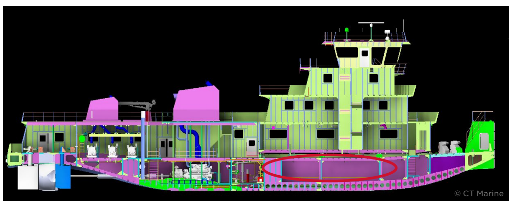
Figure 18. Rendering of internal mechanics of an inland river towboat. The placement of fuel tanks is carefully balanced to the front of the midline of the boat, with other heavy equipment located towards the stern to achieve balanced buoyancy
