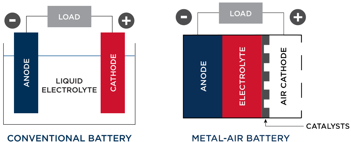
Figure 1: Conventional Battery vs Metal-Air Battery
