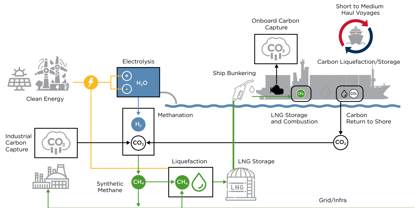
Figure 5: Case Study for CO 2 Carbon Capture on an LNG-fueled RoPax Ferry
