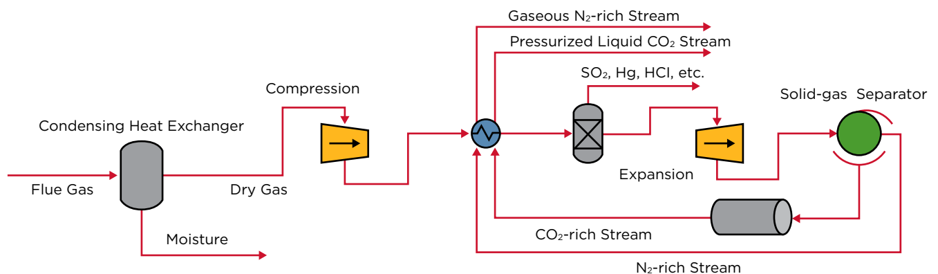
Figure 4: Typical Cryogenic Carbon Capture process
