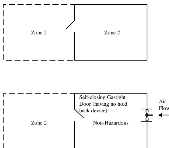
FIGURE 2 Hazardous Zones
