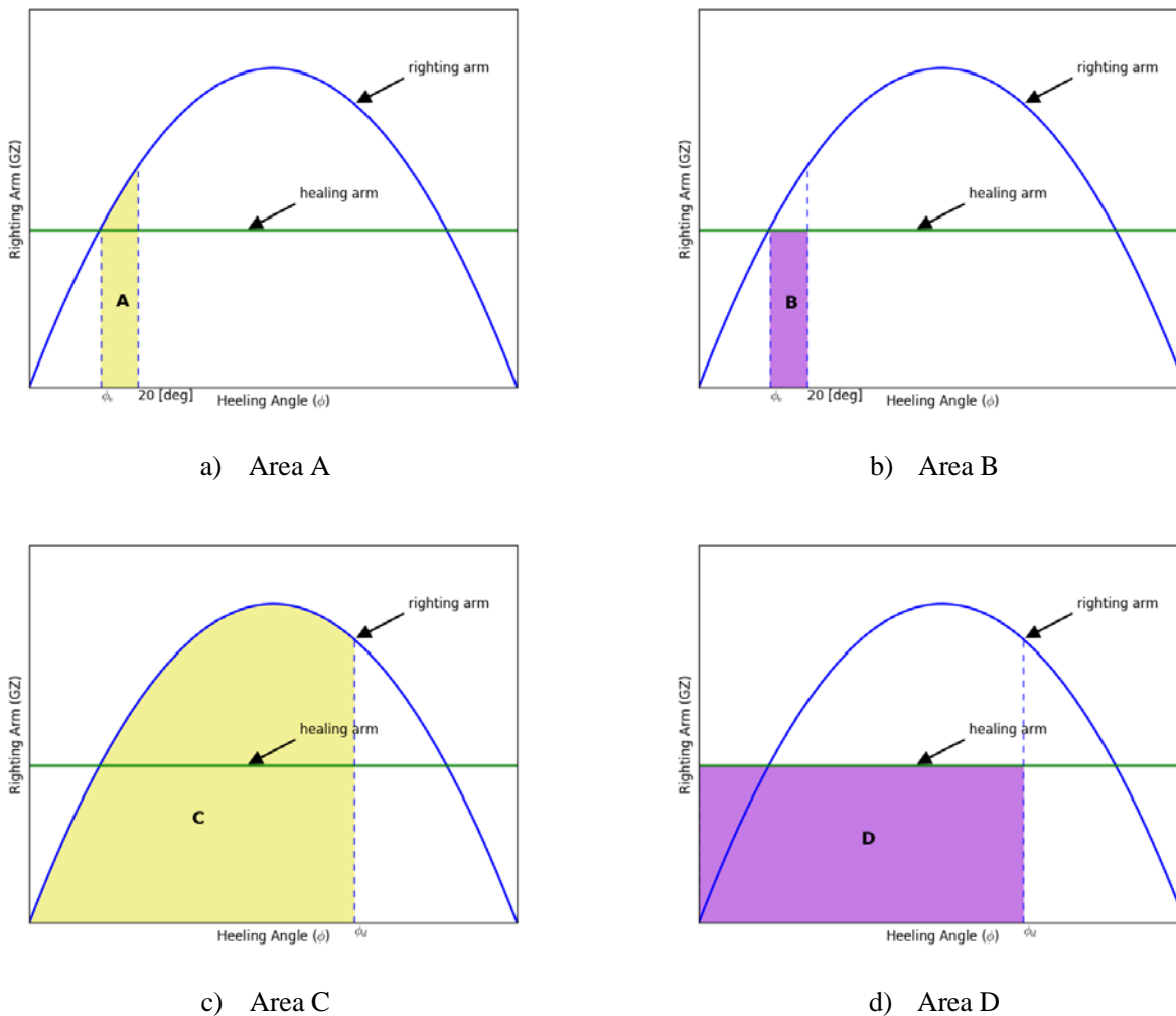
FIGURE 1 Righting Arm and Heeling Arm Curves with Areas A, B, C and D (1 July 2017)
