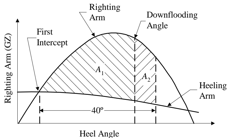
FIGURE 1 Righting Arm and Heeling Arm Curves
