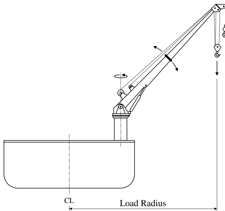
FIGURE 1 Load Radius
