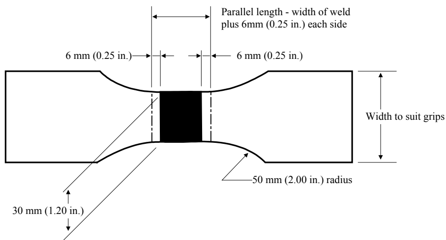
FIGURE 2 Butt Weld Tension Test Specimen
