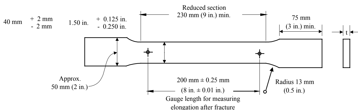
FIGURE 1 Standard Rectangular Tension Test Specimen with 200 mm (8 in.) Gauge Length
