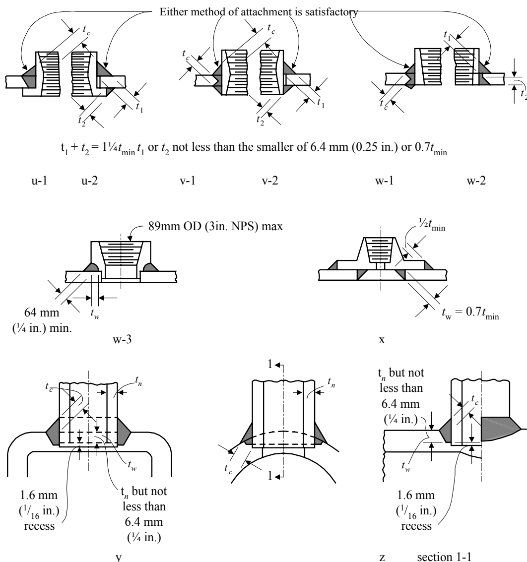
FIGURE 2 (continued) Types of Fusion-welded Construction Details
