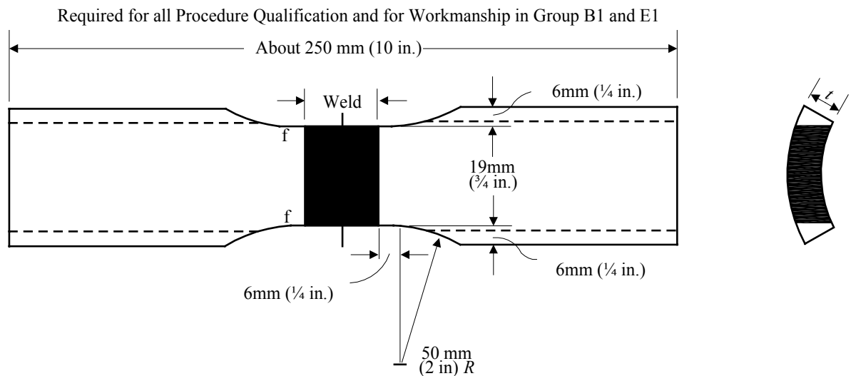
FIGURE 4 Test No. 1 – Reduced-section Tension Test for Pipe
