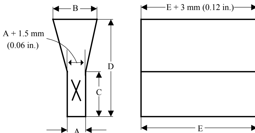
FIGURE 1 “Y” Blocks for Test Coupons
