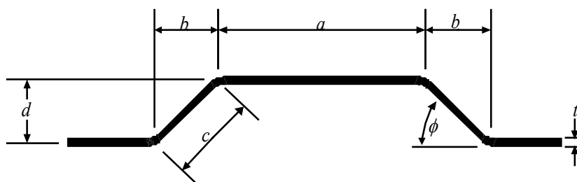
FIGURE 3 Corrugated Bulkhead
