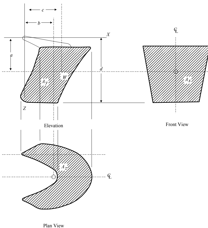
FIGURE 3 Visor Type Bow Door
