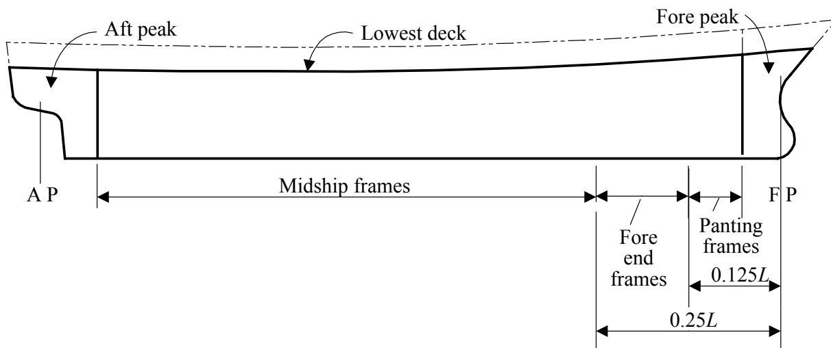
FIGURE 1 Zones of Framing
