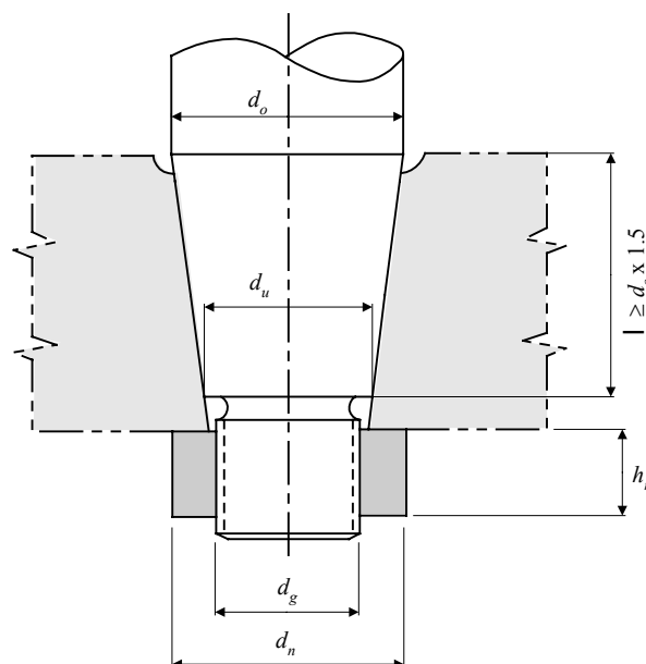
FIGURE 3 Tapered Couplings (1993)
