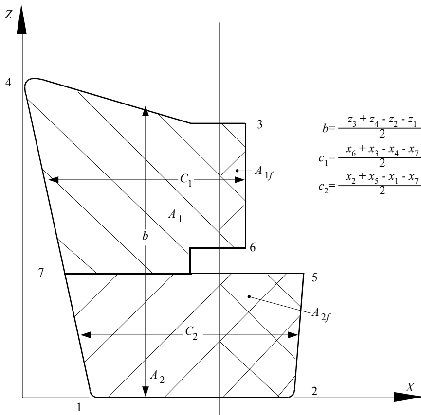
FIGURE 2 Rudder with Cutouts (1993)
