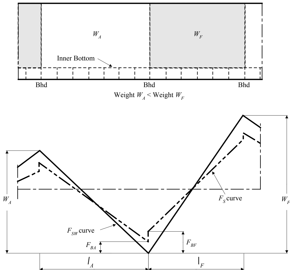
FIGURE 5 Shear Force Distribution (1997)
