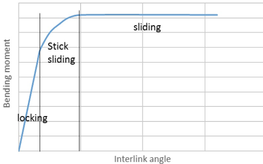
FIGURE 2 Chain Bending Moment vs Interlink Angle
