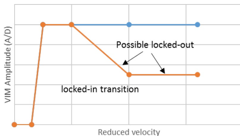
FIGURE 1 Example VIM Amplitude versus Reduced Velocity
