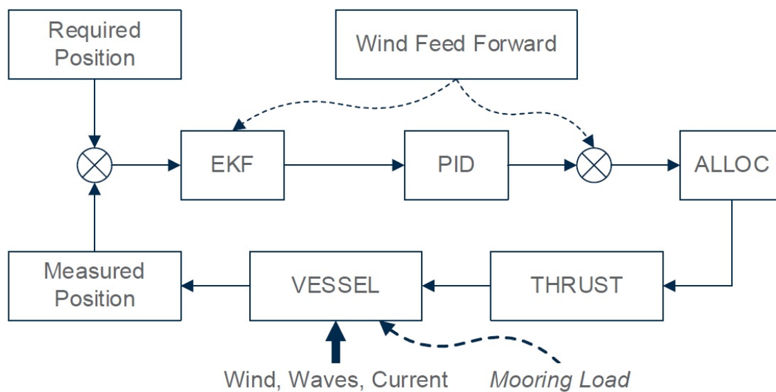
FIGURE 1 Automatic Thruster Control Feedback Loop
