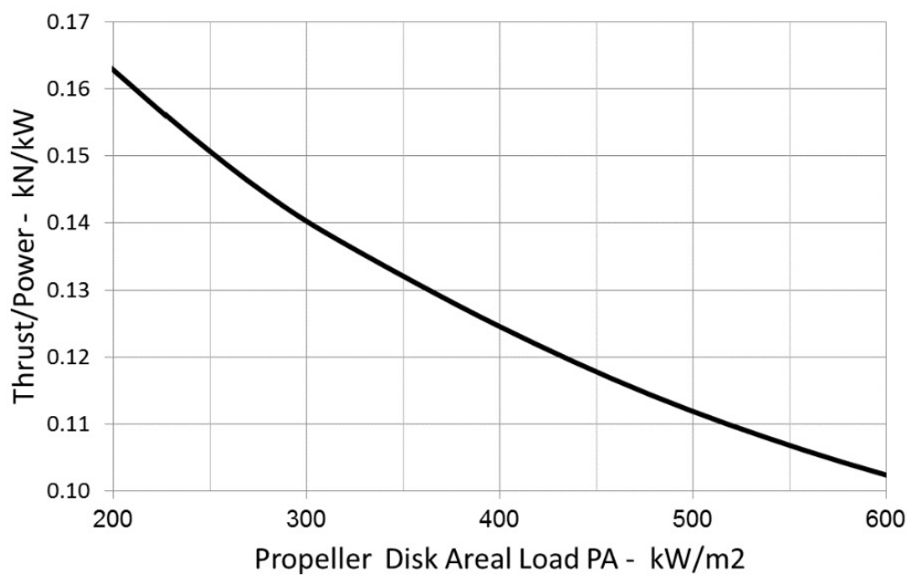
FIGURE 1 Open Propellers
