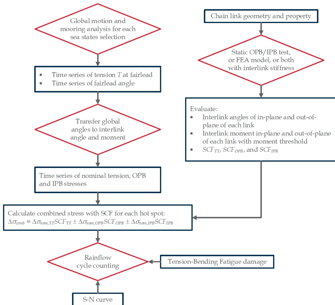
FIGURE 3 Flow Chart to Calculate OPB Fatigue Damage
