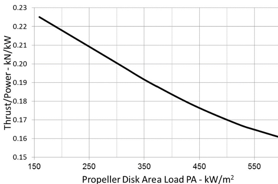
FIGURE 2 Ducted Propellers
