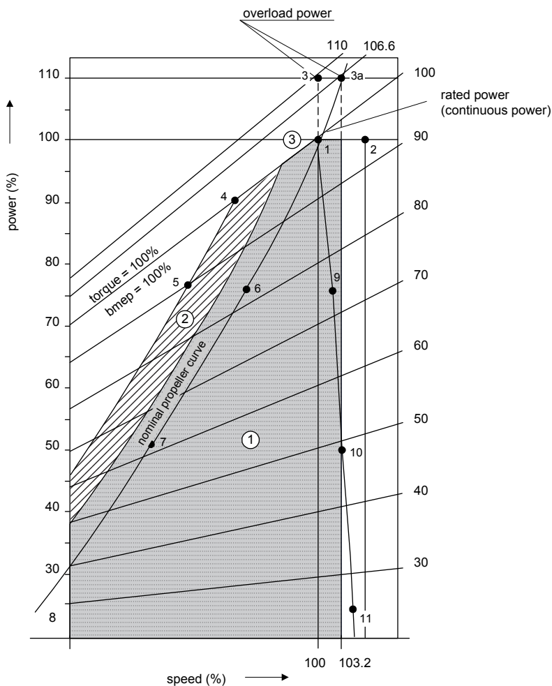
FIGURE 8 Type Test Power/Speed Diagram
