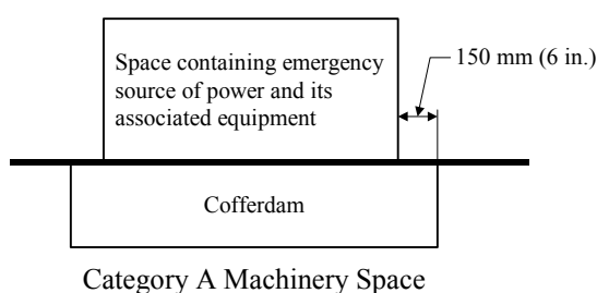
FIGURE 1 Cofferdam with Extension Beyond the Boundaries of the Space Containing the Emergency Source
