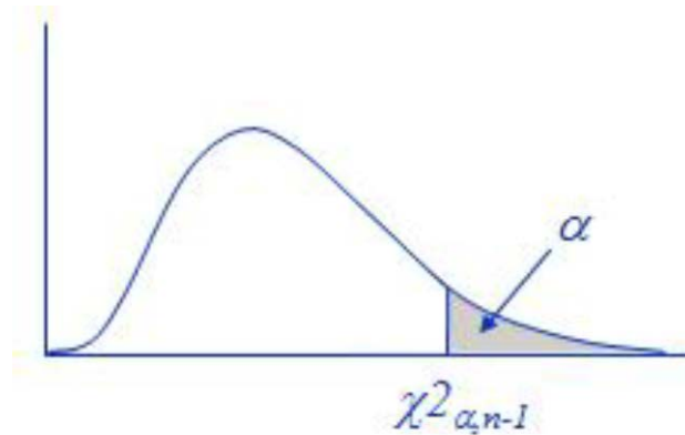
FIGURE 5 Chi-square Distribution (1 July 2018)
