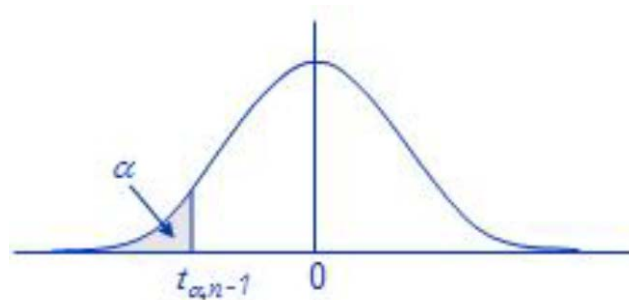
FIGURE 4 Student's t -Distribution (1 July 2018)
