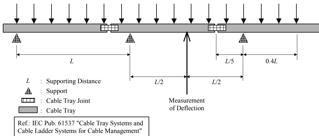
FIGURE 1 SWL Loading Test Procedure
