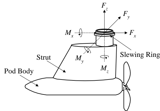
FIGURE 1 Podded Propulsion Unit
