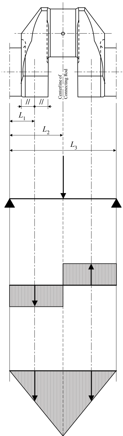
FIGURE 1 Crank Throw for In Line Engine
