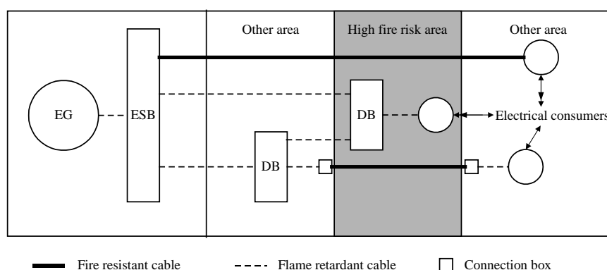
FIGURE 1 Cables within High Fire Risk Areas
