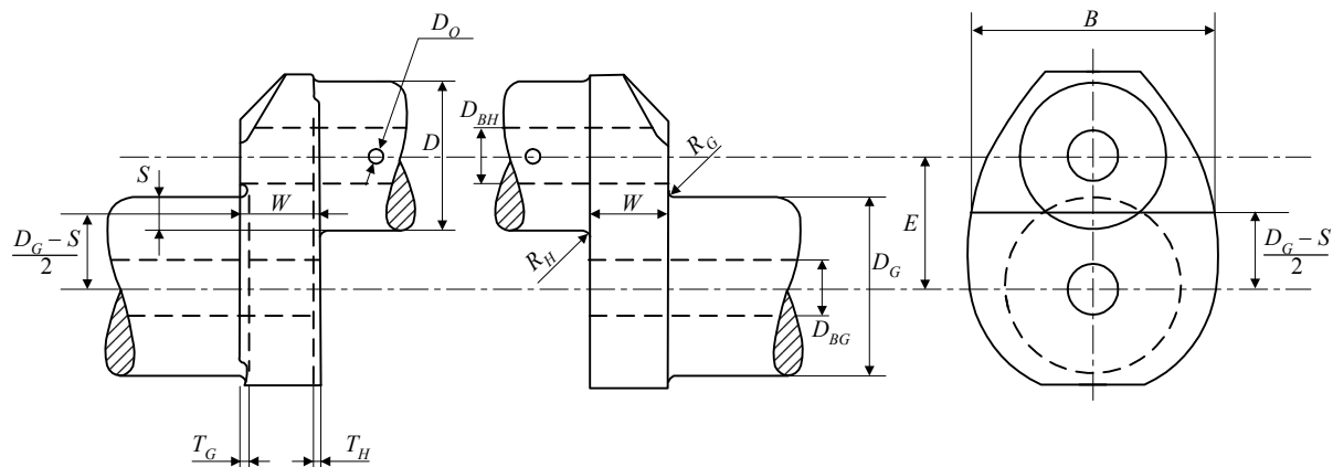
FIGURE 5 Crank Dimensions
