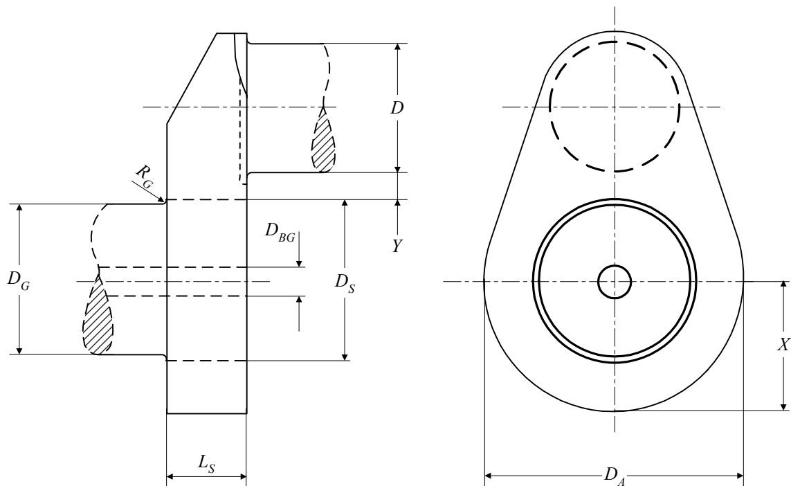
FIGURE 6 Crank Throw of Semi-built Crankshaft
