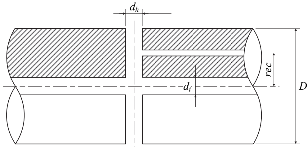
FIGURE 1 Intersection between a Radial and an Eccentric Axial Bore
