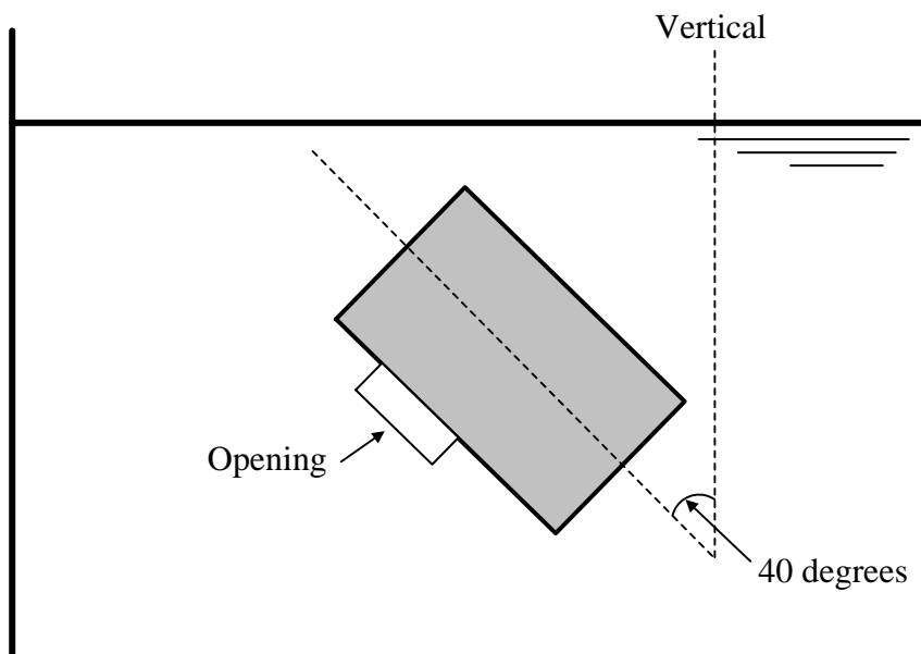
FIGURE 5 Example of Inclination 40 Degrees Opening Facing Downward
