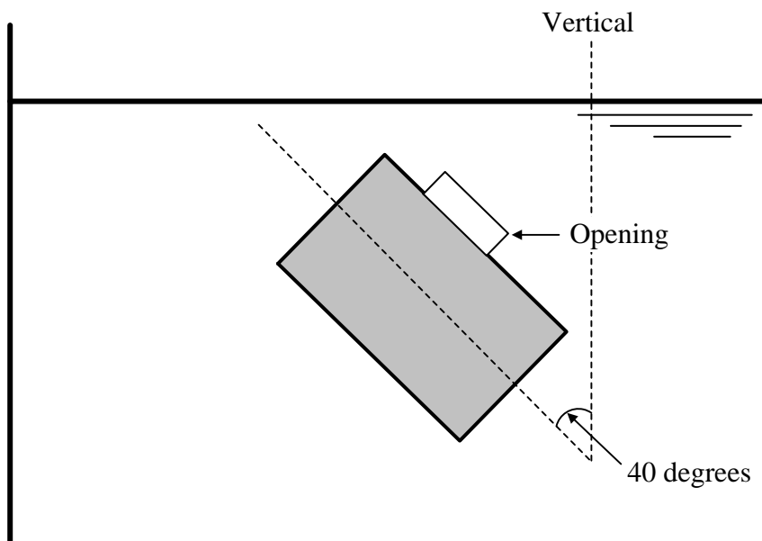
FIGURE 4 Example of Inclination 40 Degrees Opening Facing Upward
