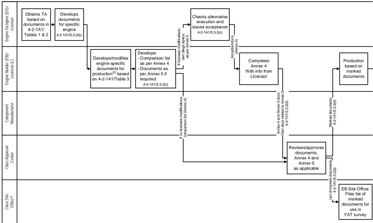
FIGURE 2 Engine Certificate Document Flow
