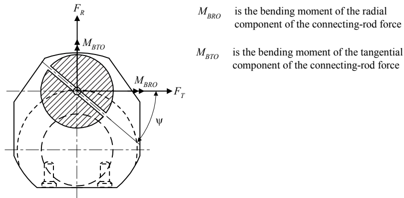
FIGURE 4 Crankpin Section Through the Oil Bore
