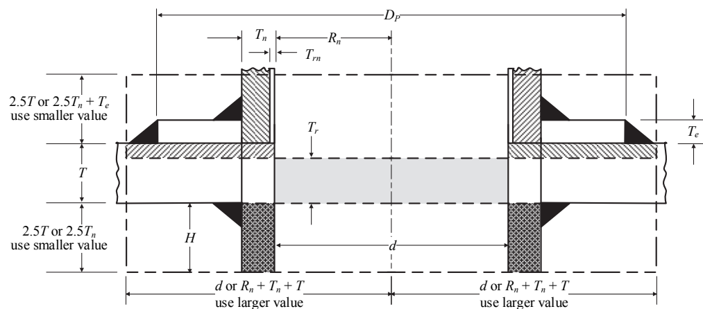
FIGURE 8 Example of Reinforced Opening
