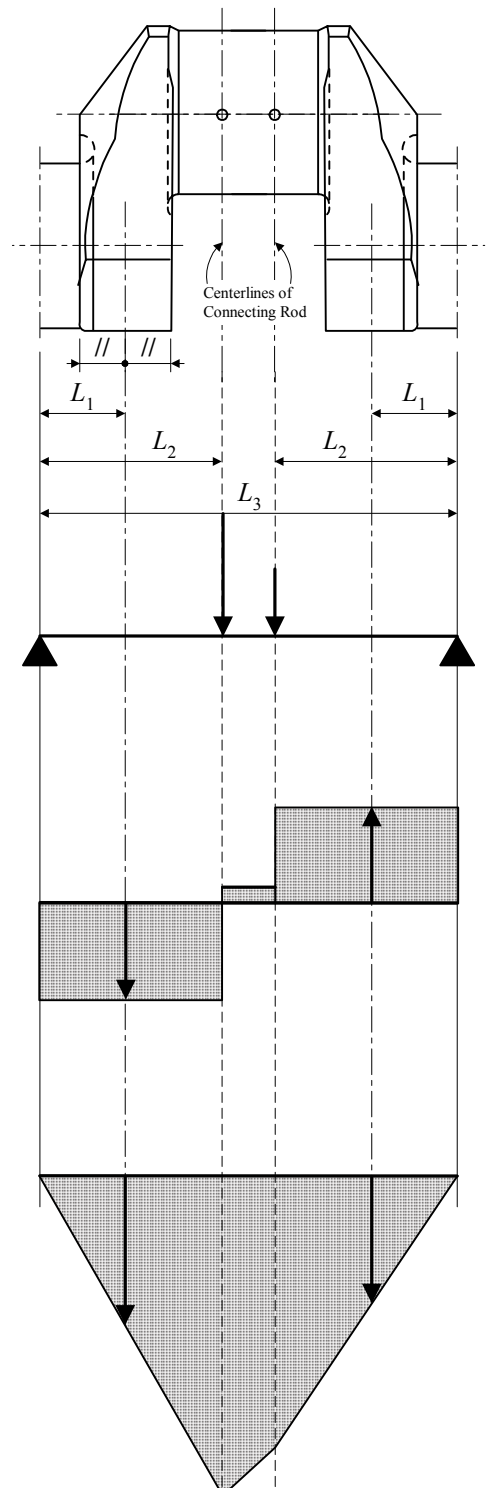
FIGURE 2 Crank Throw for Vee Engine with 2 Adjacent Connecting-Rods
