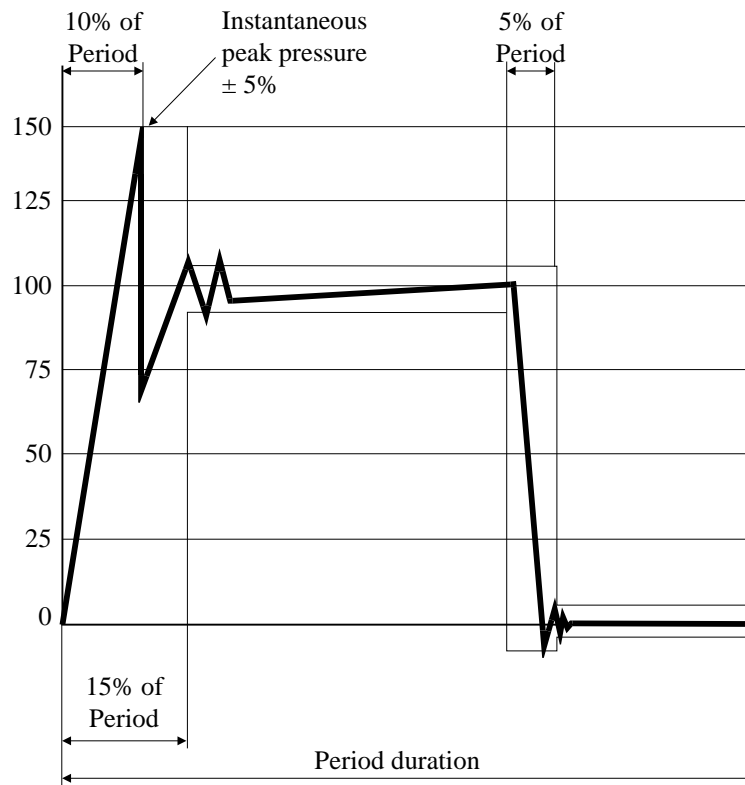
FIGURE 5 Distribution of the Pressure Pulses Magnitude % Design Pressure vs. Period Duration
