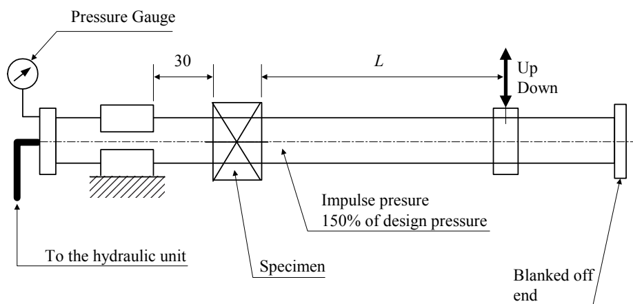
FIGURE 3 Arrangement for the Test Rig and the Joint Assembly Specimen Being Tested
