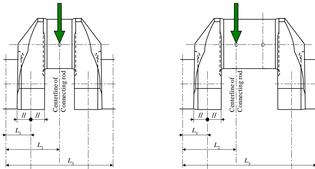
FIGURE 5 Load Applications for In-line and V-type Engines
