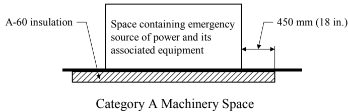
FIGURE 3 Boundary Insulated to A-60 with the Insulation Extending Beyond the Boundaries of the Space Containing the Emergency Source
