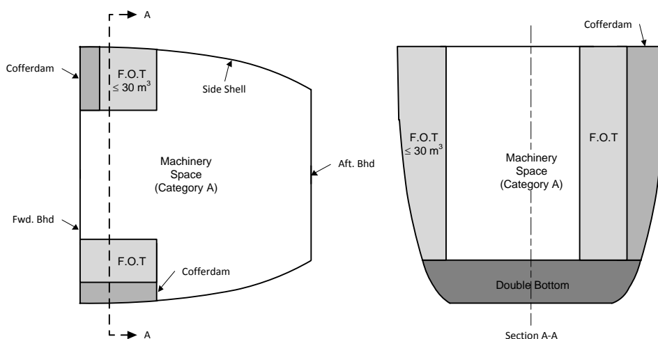
FIGURE 7 Acceptable Fuel Oil Tanks Arrangements Inside Category A Machinery Spaces
