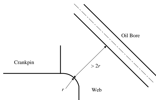
FIGURE 1 Oil Bore Proximity to Fillet
