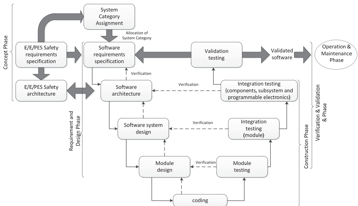
FIGURE 1 V-Model for SDLC
