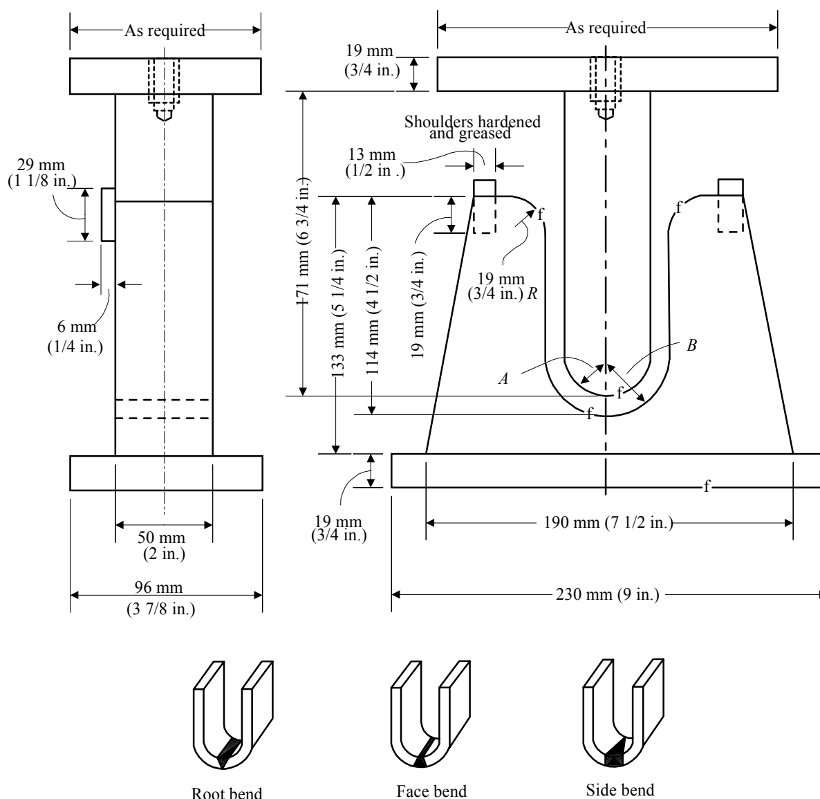
FIGURE 7 Guided Bend Test Jig
