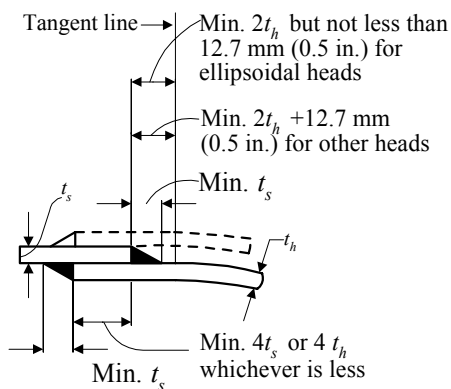
a Single fillet lap weld
