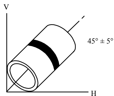
d Inclined fixed (6G) 9
