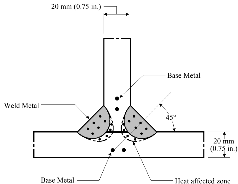
FIGURE 4 Fillet Weld Hardness Test Locations
