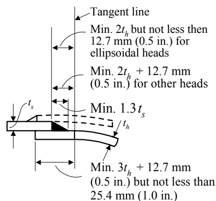
a Single fillet lap weld
