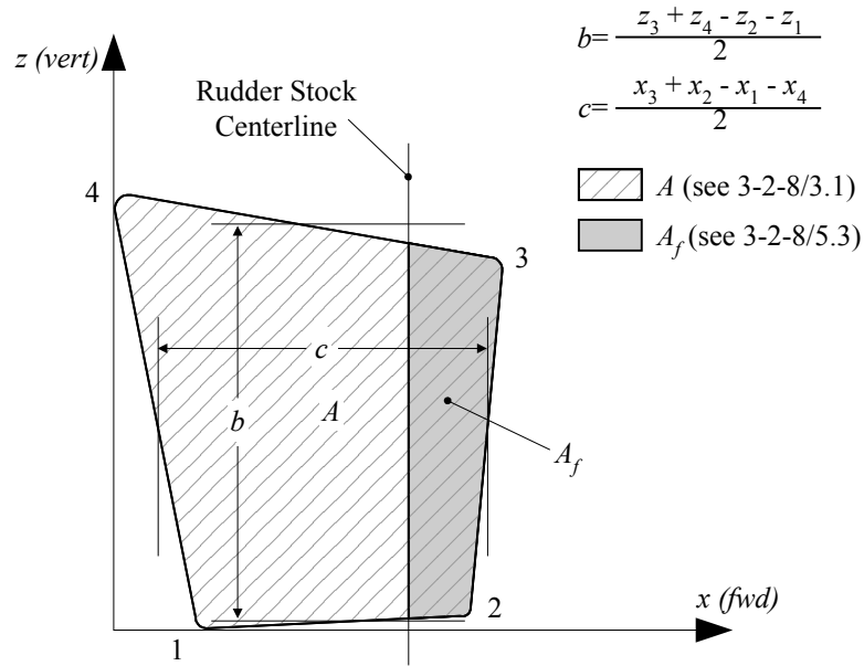
FIGURE 1 Rudder Blade without Cutouts
