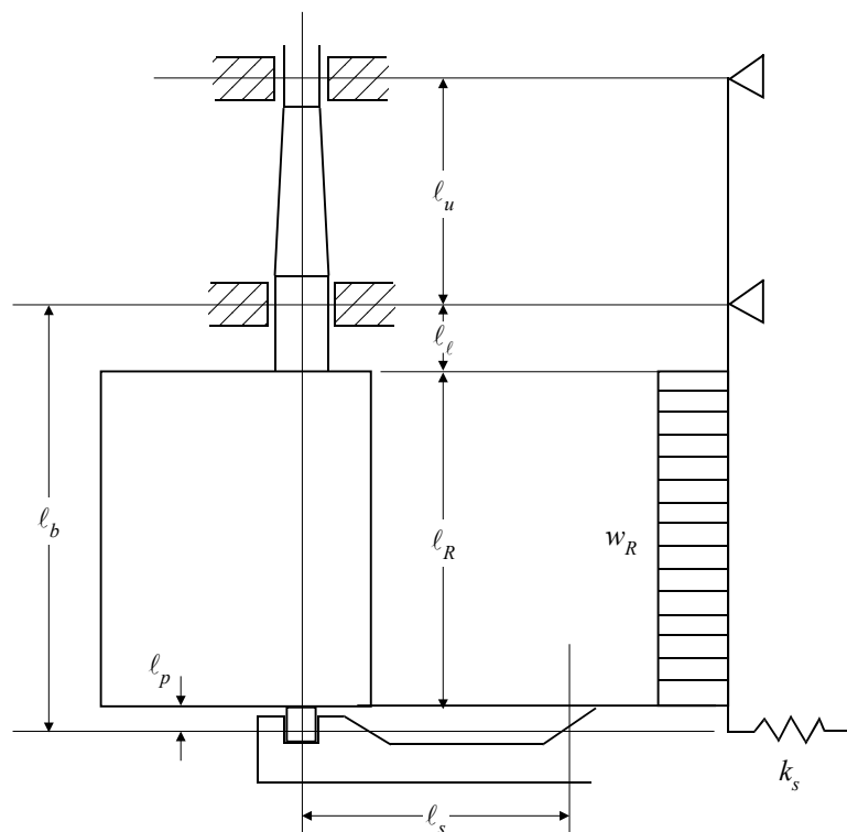
FIGURE 2 Rudder Supported by Shoe Piece
