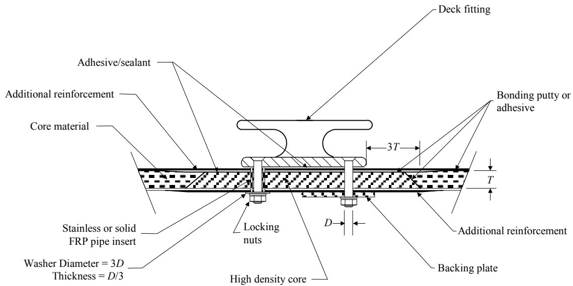
FIGURE 7 Deck Fittings
