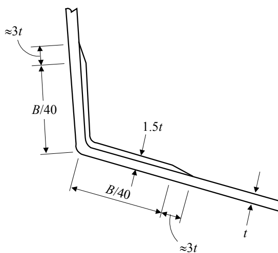
FIGURE 14a Chine or Transom – Single Skin Construction
