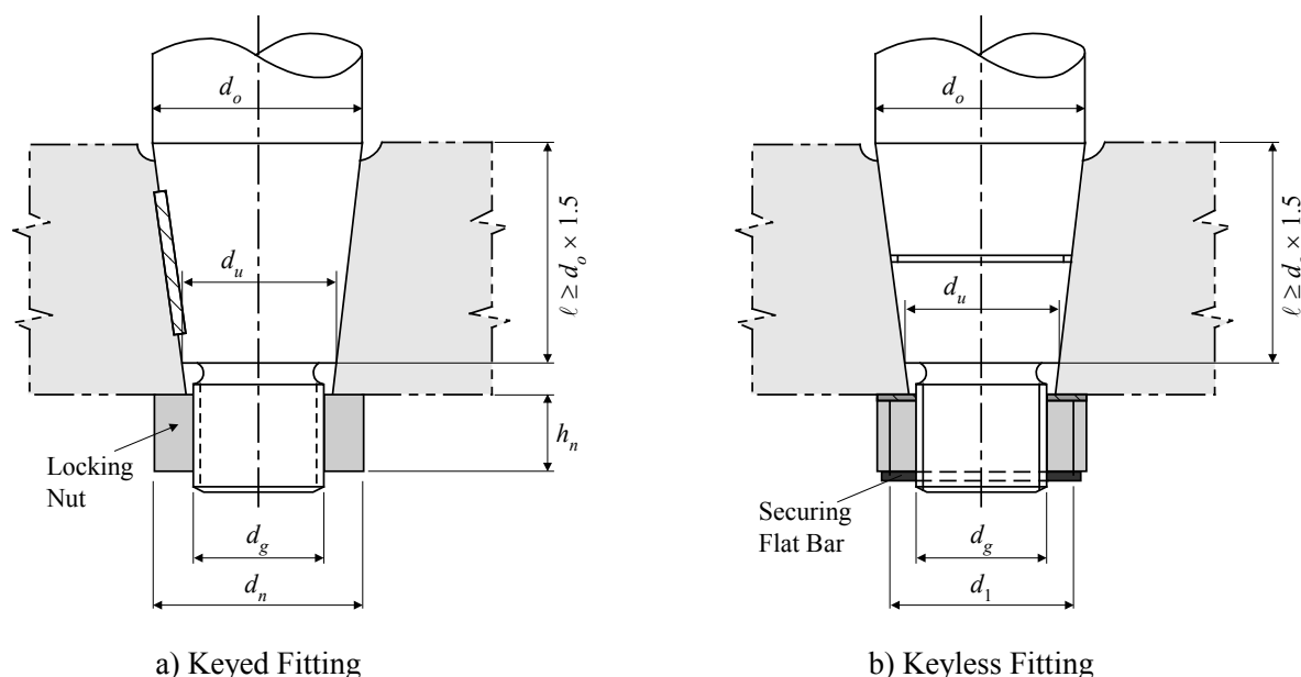
FIGURE 3 Tapered Couplings
