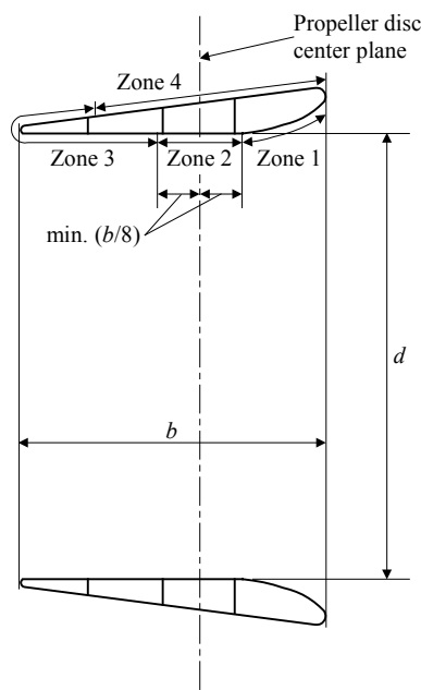
FIGURE 1 Propeller Nozzle Section View
