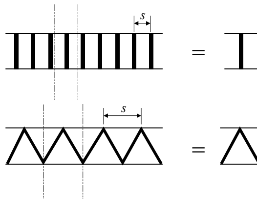
FIGURE 2 Extruded Planking
