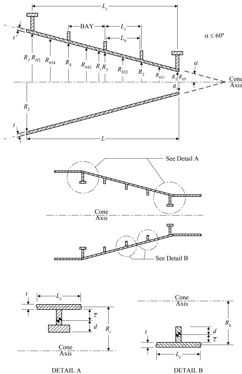
FIGURE 5 Definitions – Cones
