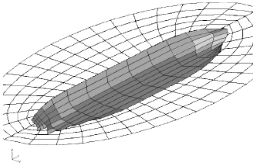
Figure 29. Panelization for the 300,000 ton tanker
