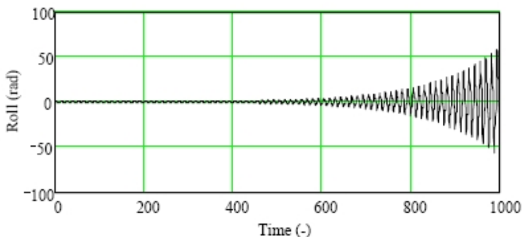
Figure 17. Numerical solution of roll equation (9) with \bar{\omega}_m = 0.558 \bar{\omega}_a = 0.609 and damping set to damping threshold with formula (32) \mu_T = 0.1559 (data are based on simplified method)
