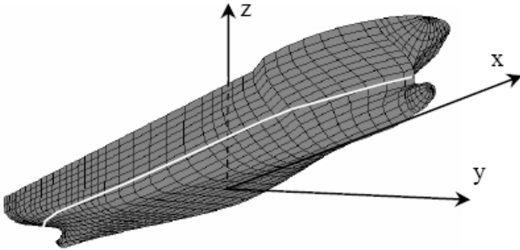
Figure 9. Coordinate system for hydrostatic calculations
