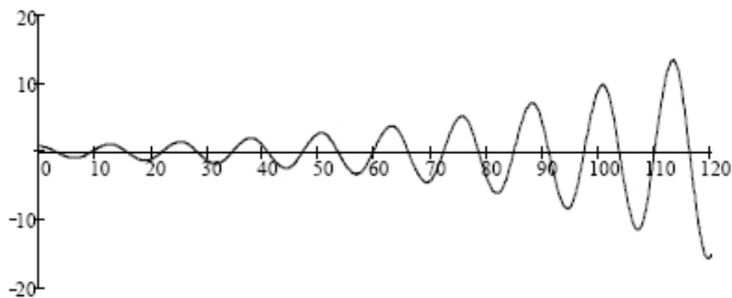
Figure 5. Sample of parametric roll (parametric resonance)
