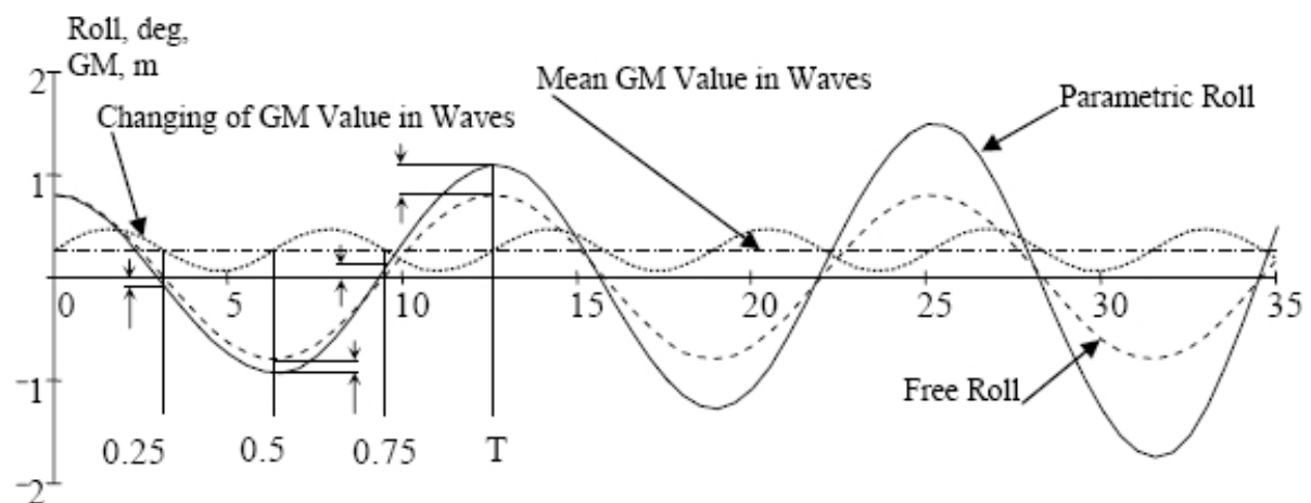
Figure 6. Development of parametric roll
