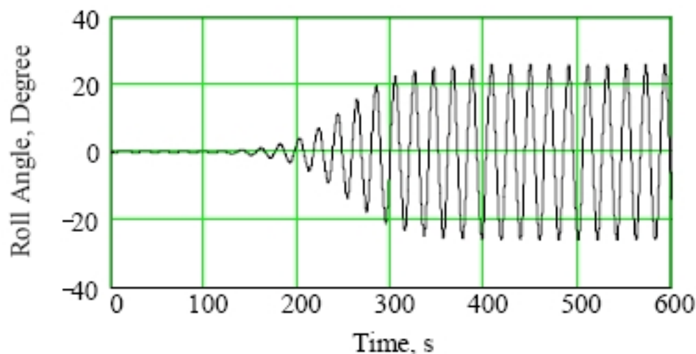
Figure 34. Development of parametric roll in regular waves (wave amplitude 4.2 m, frequency 0.485 \text{ s}^{-1} , speed 10 knots)
