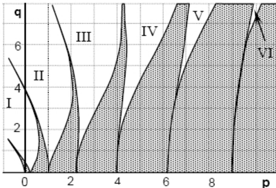
Figure 14. Ince-Strutt diagram
