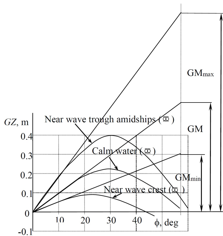
FIGURE 2 Change of Stability in Longitudinal Wave
