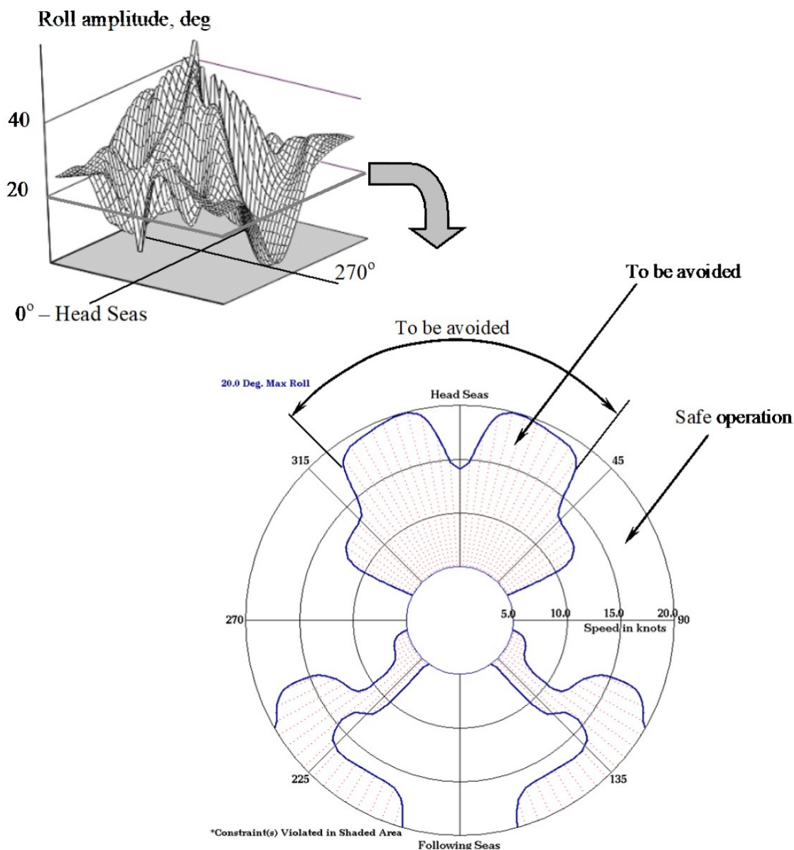
FIGURE 1 Sample Polar Diagram
