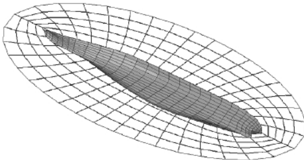
Figure 19. Geometry of C11 class container carrier
