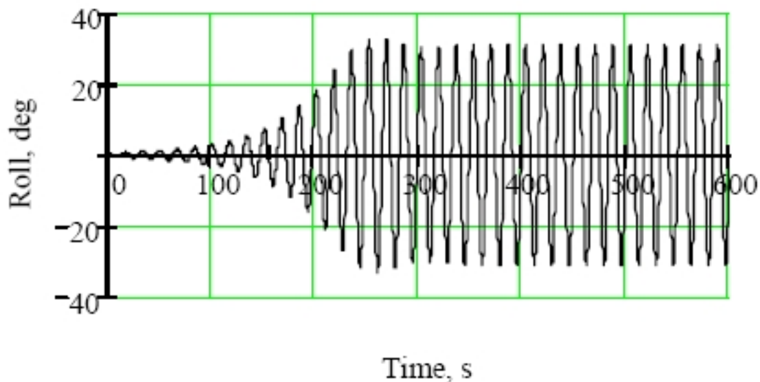
Figure 37. Result of numerical integration of rolling equation (50)
