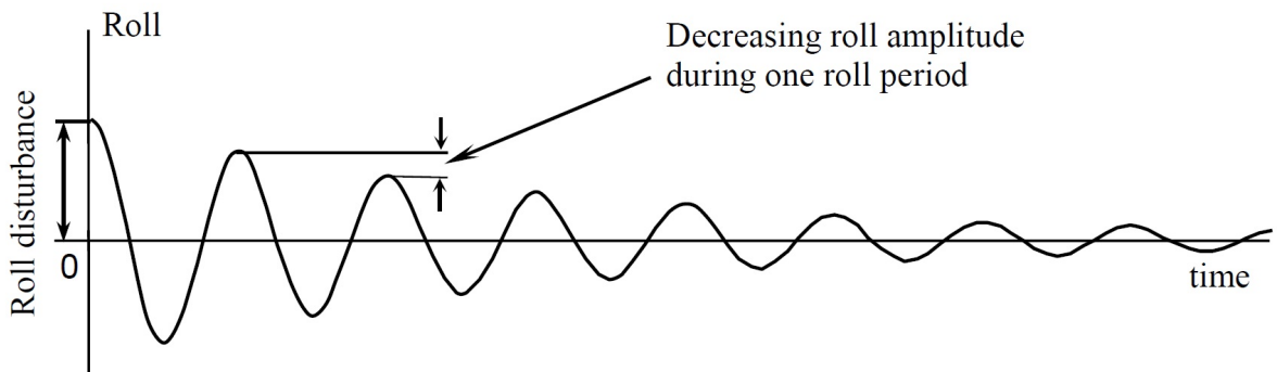
FIGURE 7 Successively Decreasing Roll Amplitudes due to Roll Damping in Calm Water
