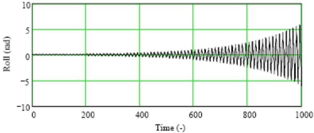
Figure 18. Numerical solution of roll equation (9) with \varpi_m = 0.574 \varpi_a = 0.581 and damping set to damping threshold with formula (32) \mu_T = 0.132 (data are based on EUREKA)
