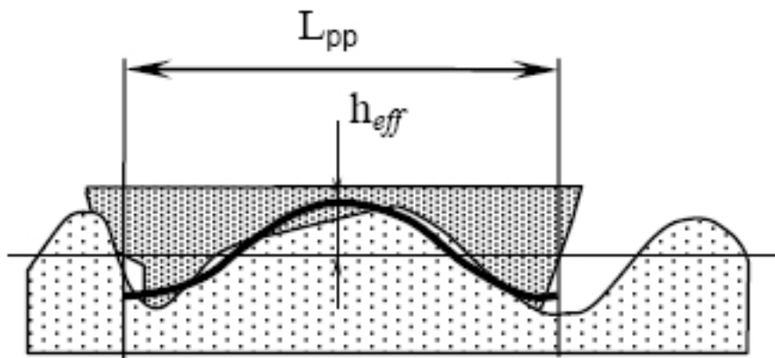
Figure 42. Concept of effective wave [Grim, 1961]
