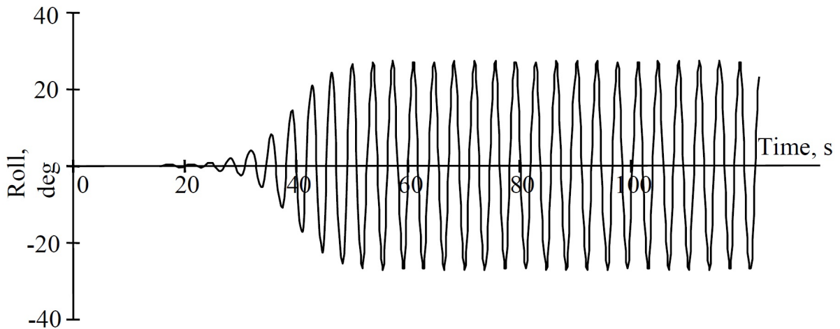
FIGURE 9 Development of Parametric Roll
