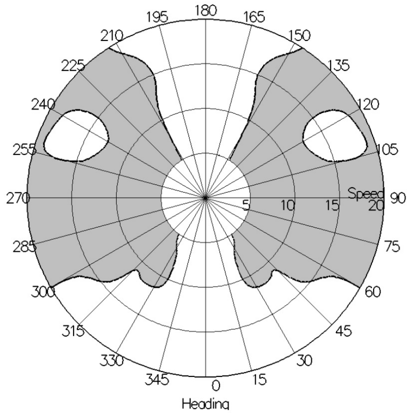
FIGURE 5 Sample Polar Diagram –Partial Load, Sea State 9
