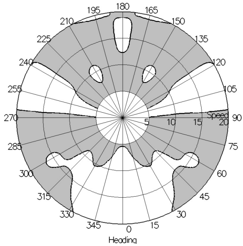
FIGURE 2 Sample Polar Diagram –Full Load, Sea State 9
