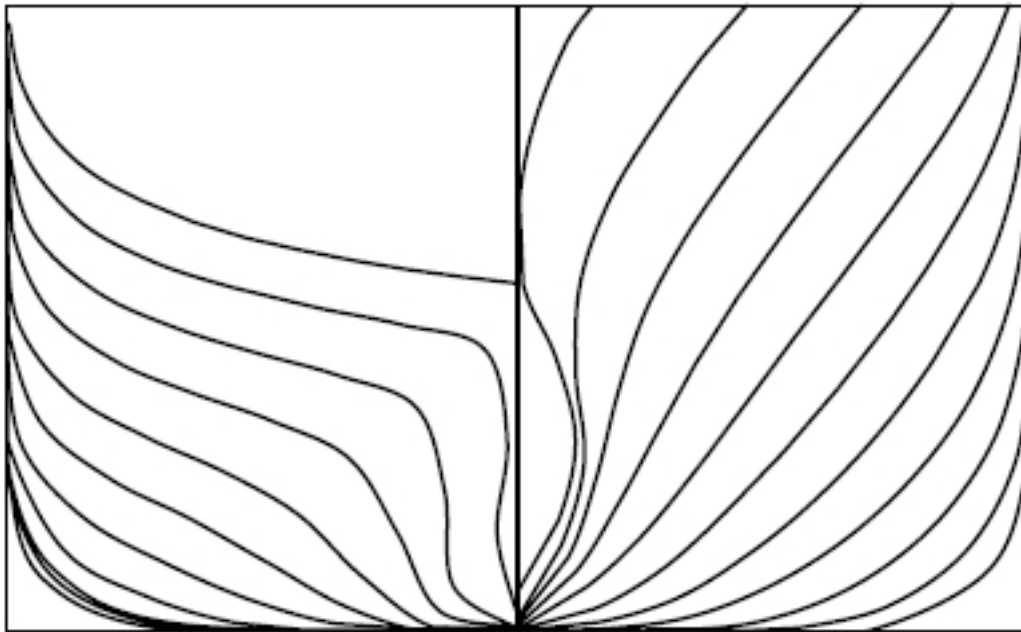
Figure 8. Lines of Post-Panamax C11 class container carrier
