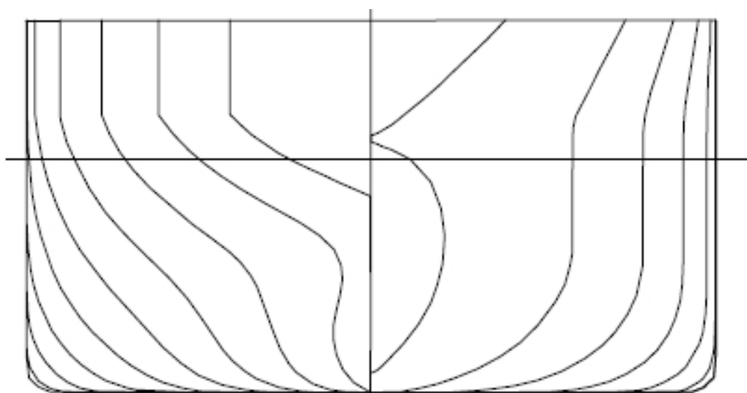
Figure 26. Lines of 300,000-ton tanker
