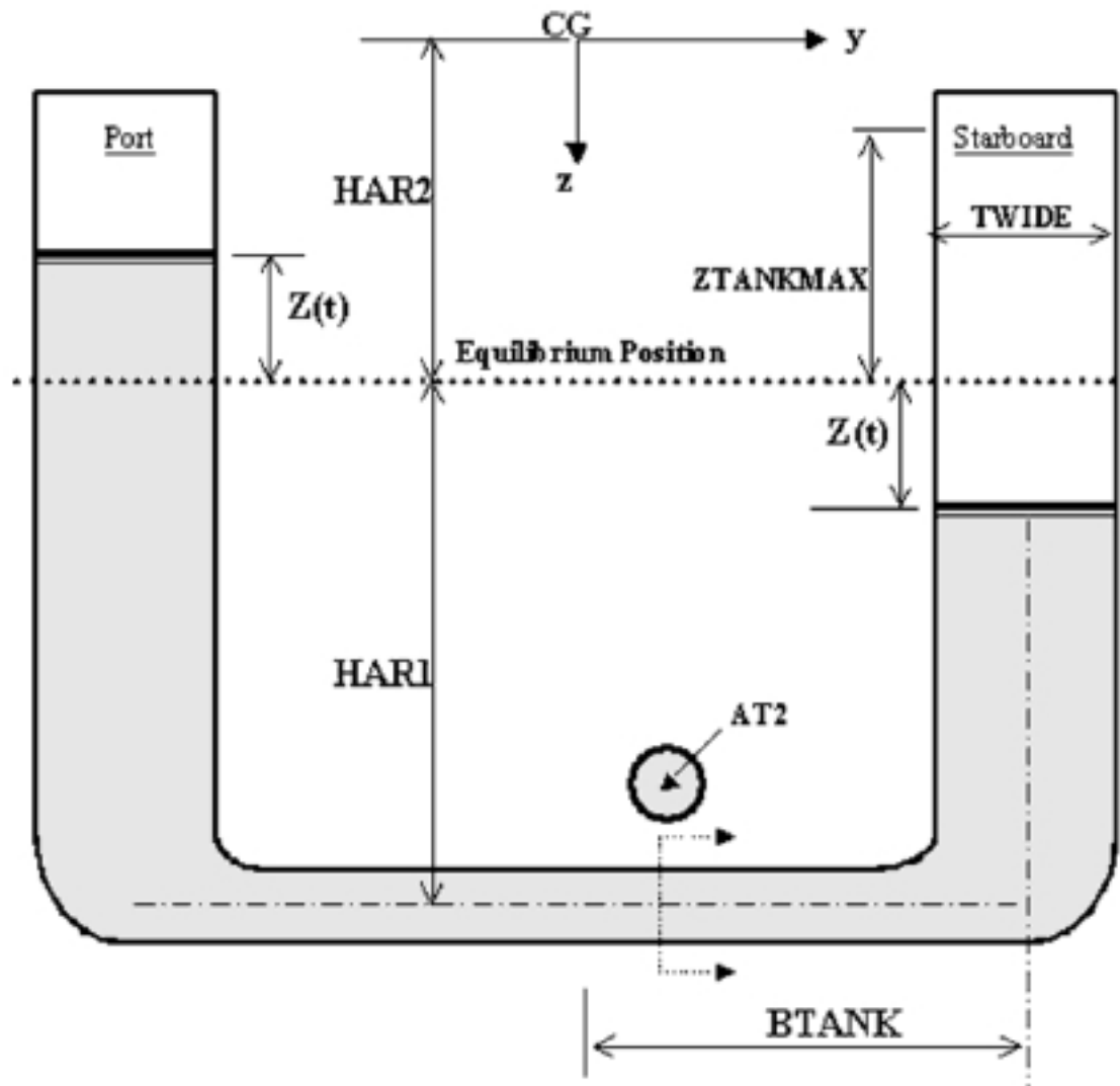
Figure 44. Schematic of an anti-roll tank
