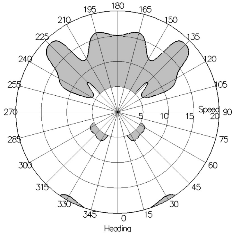
FIGURE 4 Sample Polar Diagram –Full Load, Sea State 7
