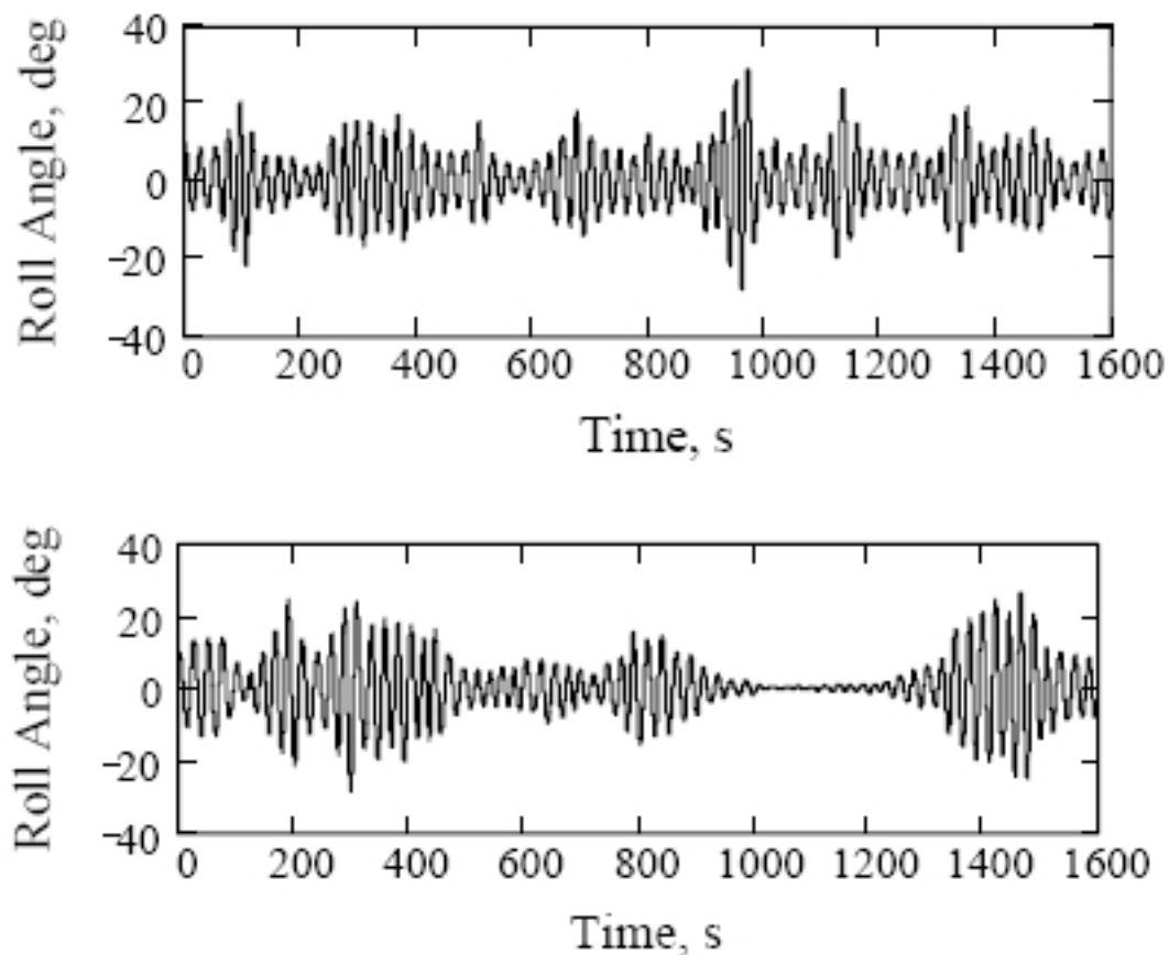
Figure 38. Sample of two parametric realizations
