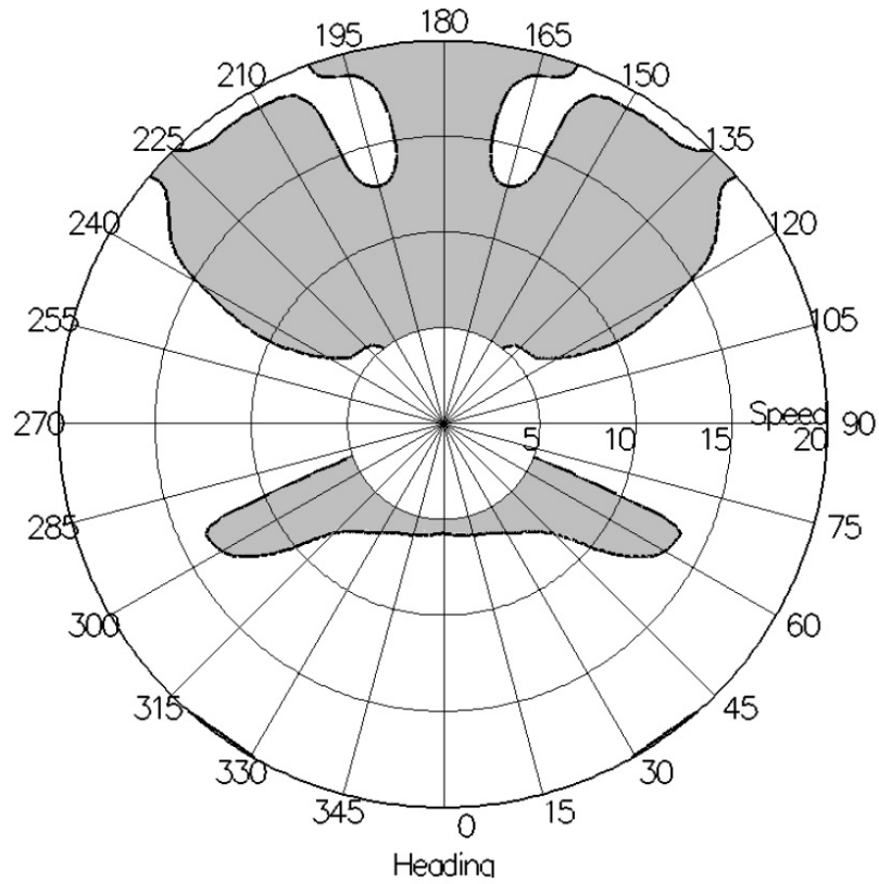
FIGURE 3 Sample Polar Diagram –Full Load, Sea State 8
