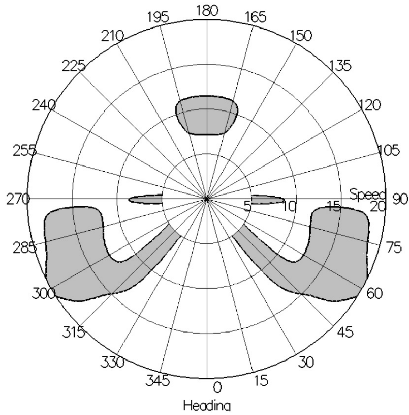
FIGURE 7 Sample Polar Diagram –Partial Load, Sea State 7
