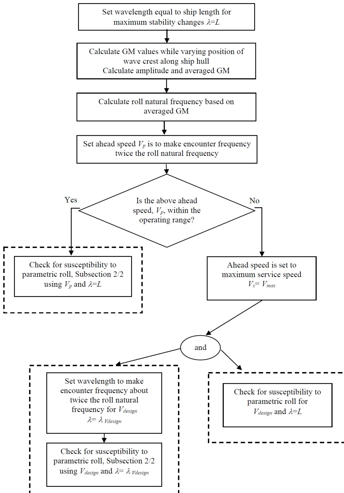
FIGURE 1 Diagram Showing Selection of Wavelength and Ahead Speed (1 August 2024)
