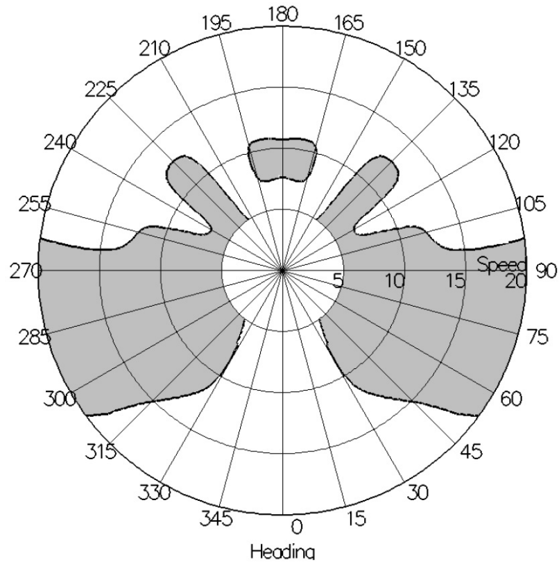
FIGURE 6 Sample Polar Diagram –Partial Load, Sea State 8
