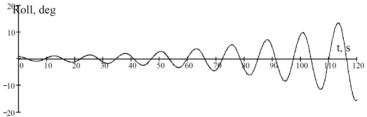
FIGURE 4 Parametric Roll Resonance
