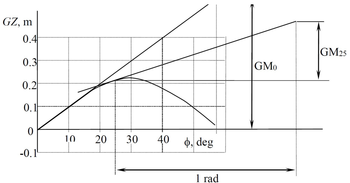
FIGURE 8 Change of Instantaneous GM Value with Increasing Heel Angle
