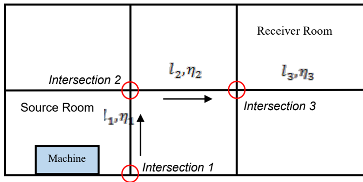
FIGURE 4 Structure-borne Sound Transmission Path in Ships and Offshore Units (1 April 2019)
