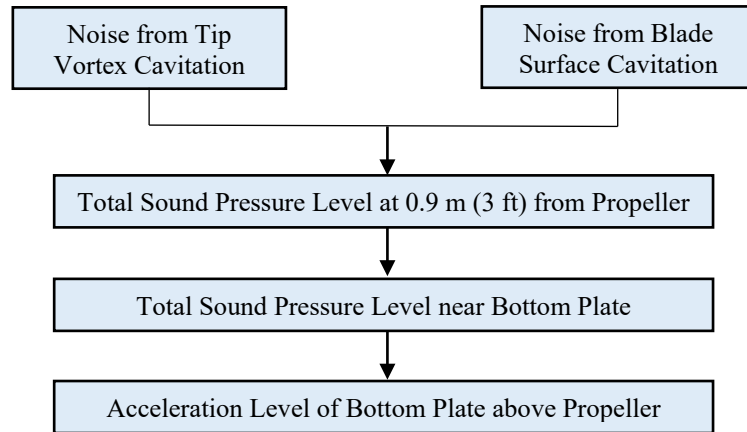
FIGURE 4 Calculation Procedure for Ship Propeller Induced Vibration (1 April 2019)
