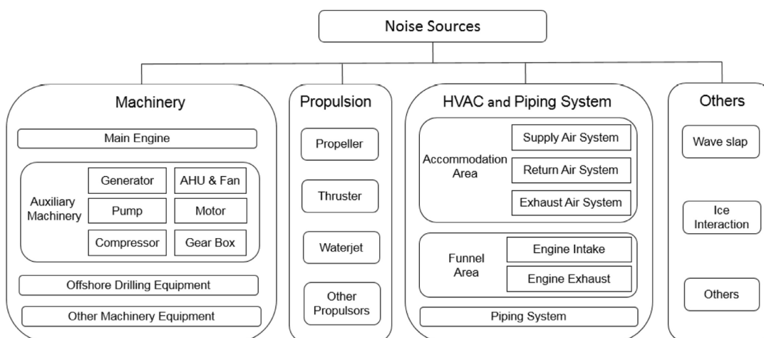
FIGURE 2 Noise Sources On Board Ships and Offshore Units (1 April 2019)
