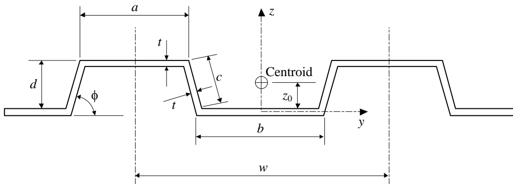
FIGURE 2 Corrugated Bulkhead
