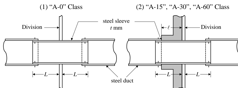
FIGURE 1 Ventilation Ducts Penetrating “A” Class Divisions
