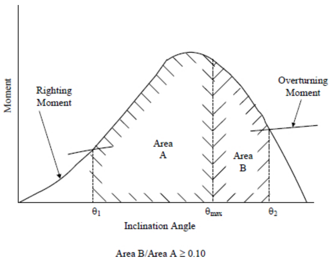
FIGURE 5 Capsize Criterion
