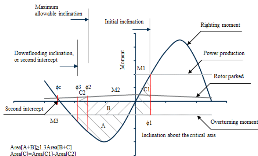
FIGURE 4 Intact Stability Curve for the RNA after Loss of Thrust Force – Heel in the Opposite Direction of Wind (2024)
