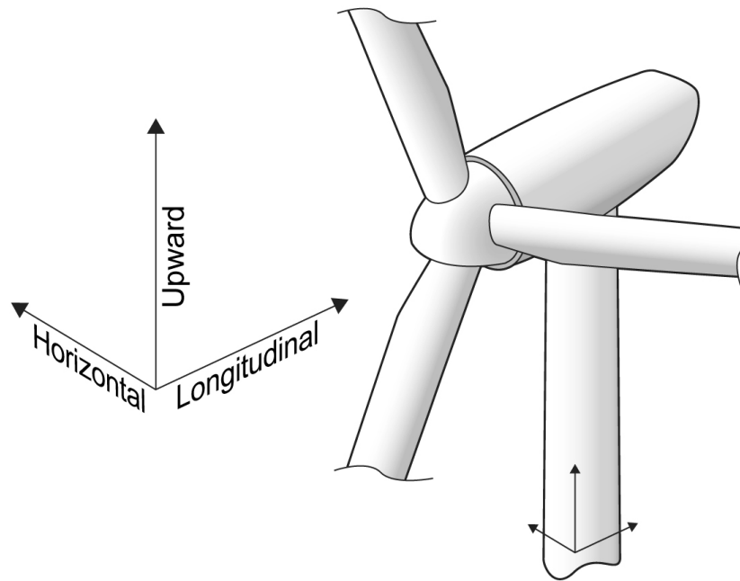
FIGURE 1 Vector Components of Turbulent Wind Velocity (2024)
