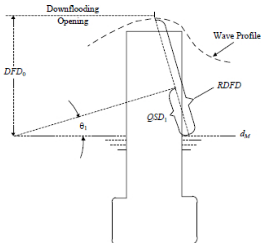
FIGURE 6 Downflooding Criterion
