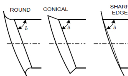
FIGURE 13 Tunnel Configuration
