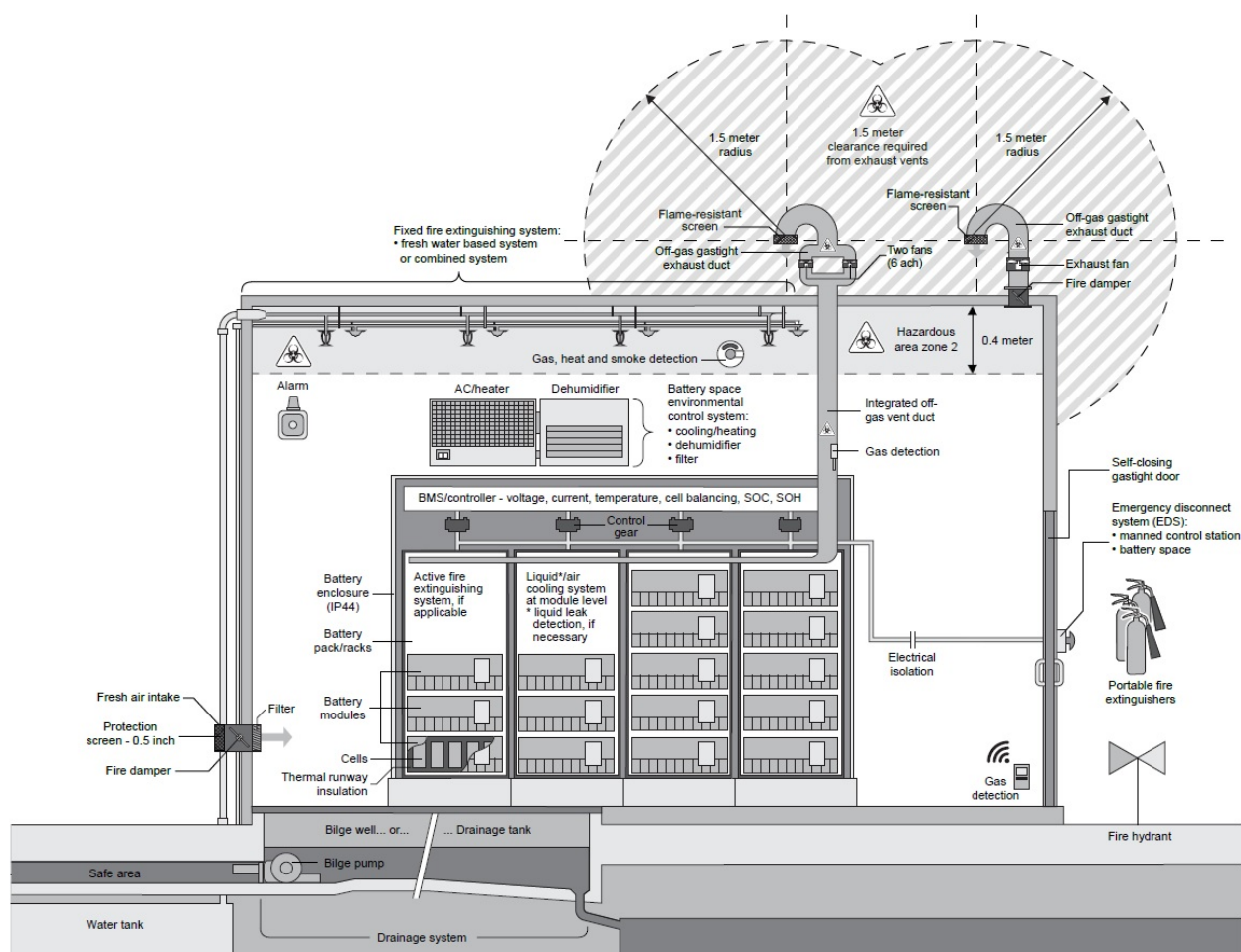
FIGURE 2 Design 2 with Integrated Off-Gas Vent (1 December 2025)
