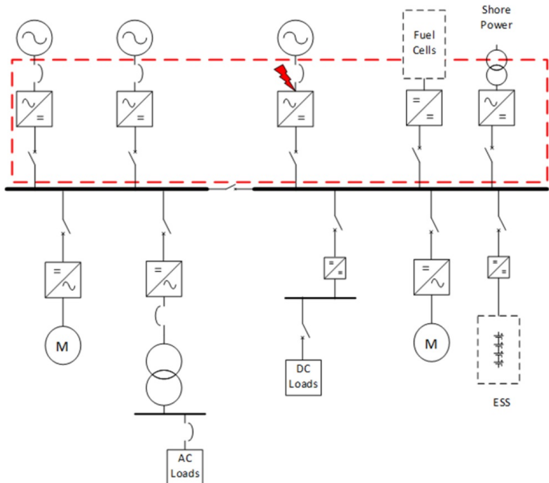
FIGURE 2 Short Circuit Fault Location 1 – Upstream of DC Bus (example schematic for reference only)
