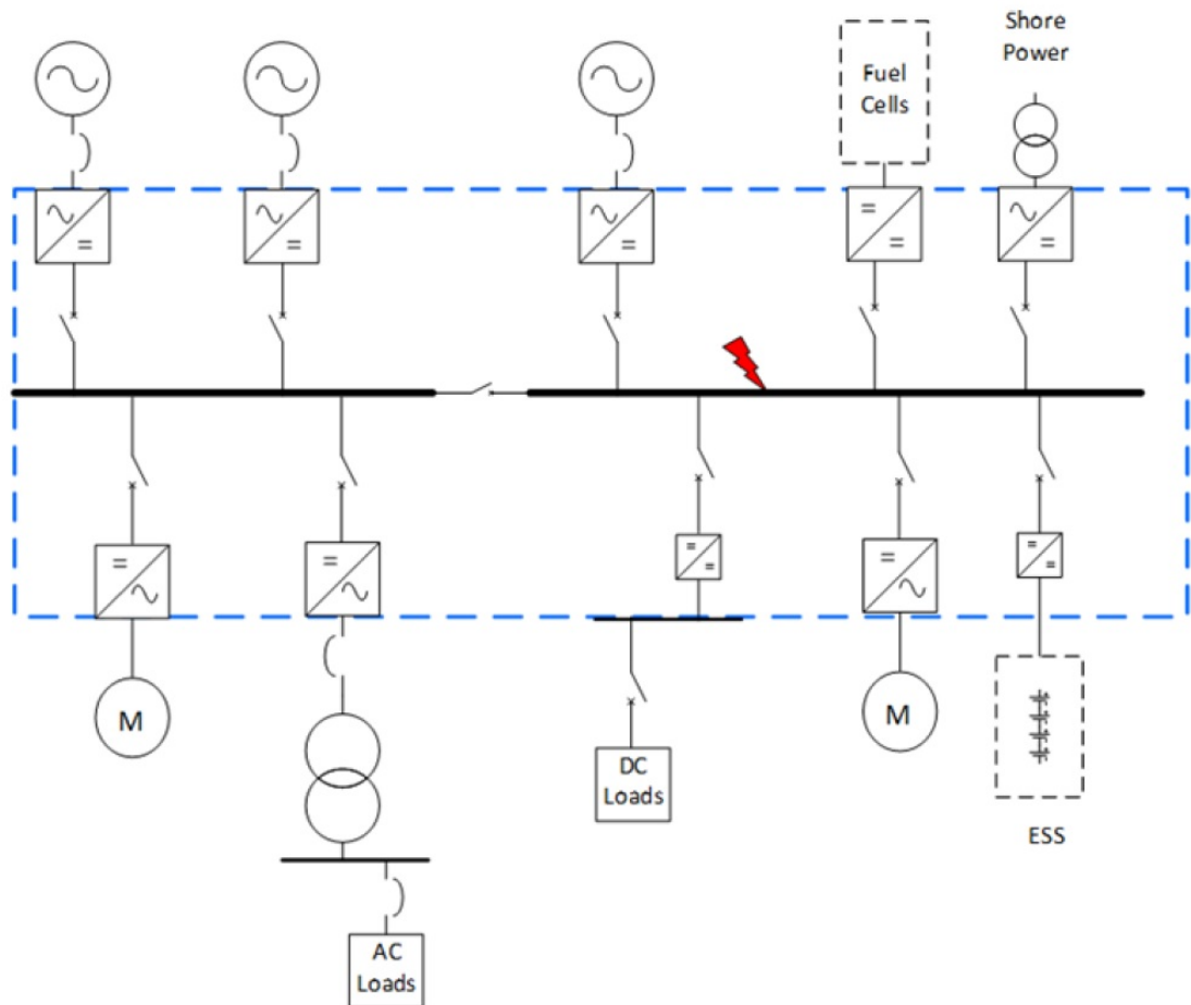
FIGURE 3 Short Circuit Fault location 2 – On DC Bus (example schematic for reference only)
