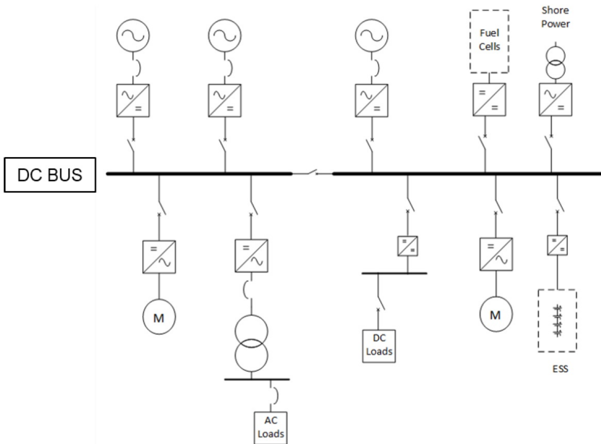
FIGURE 1 Example of a DC Power Distribution System
