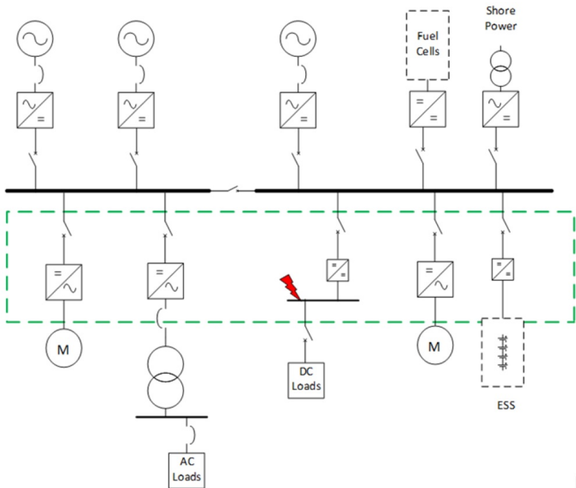
FIGURE 4 Short Circuit Fault Location 3 – Downstream of DC Bus (example schematic for reference only)
