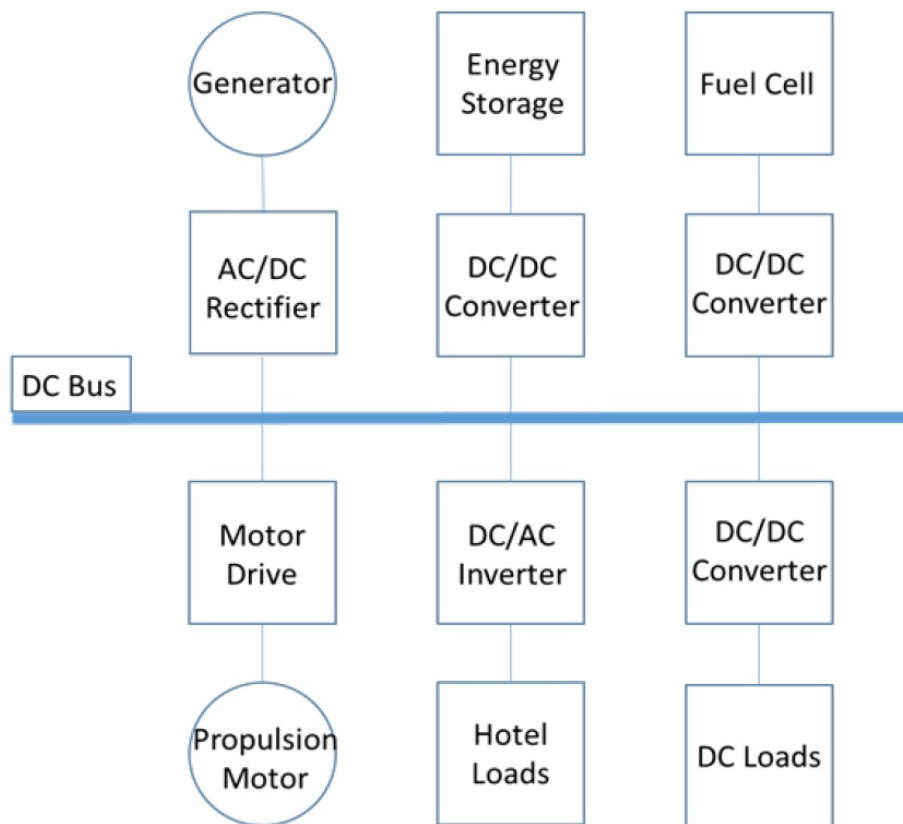
FIGURE 1 Example of a DC Power Distribution System Block Diagram Concept
