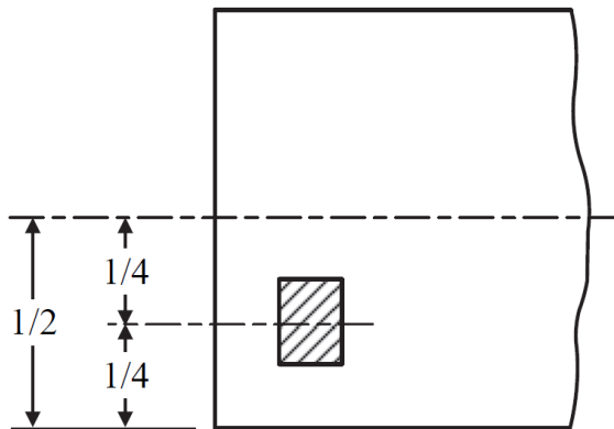
FIGURE 2 Position of the Test Samples – Bulb Flats
