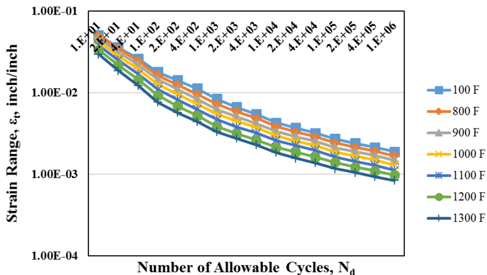
FIGURE 1 Design Fatigue Strain Range, \epsilon_p , for 304 Stainless Steel (1,2)
