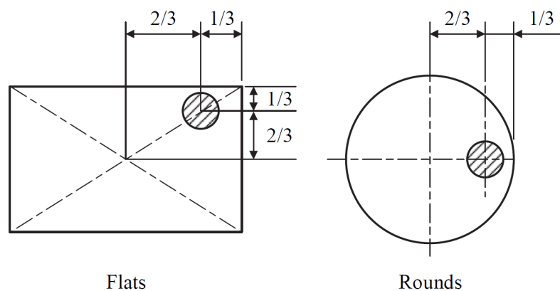
Flats and rounds (bars)
