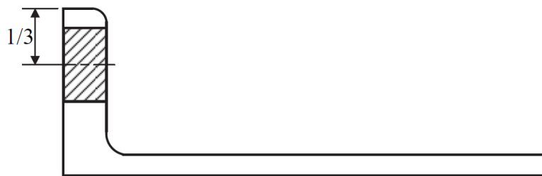
FIGURE 5 Position of the Test Samples – Channels and Beams
