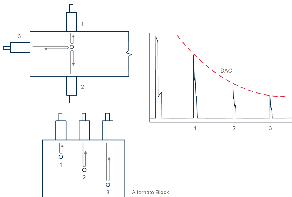
FIGURE 4 Compression Wave Sensitivity Calibration
