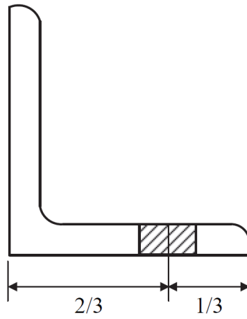
FIGURE 4 Position of the Test Samples – Unequal Angles
