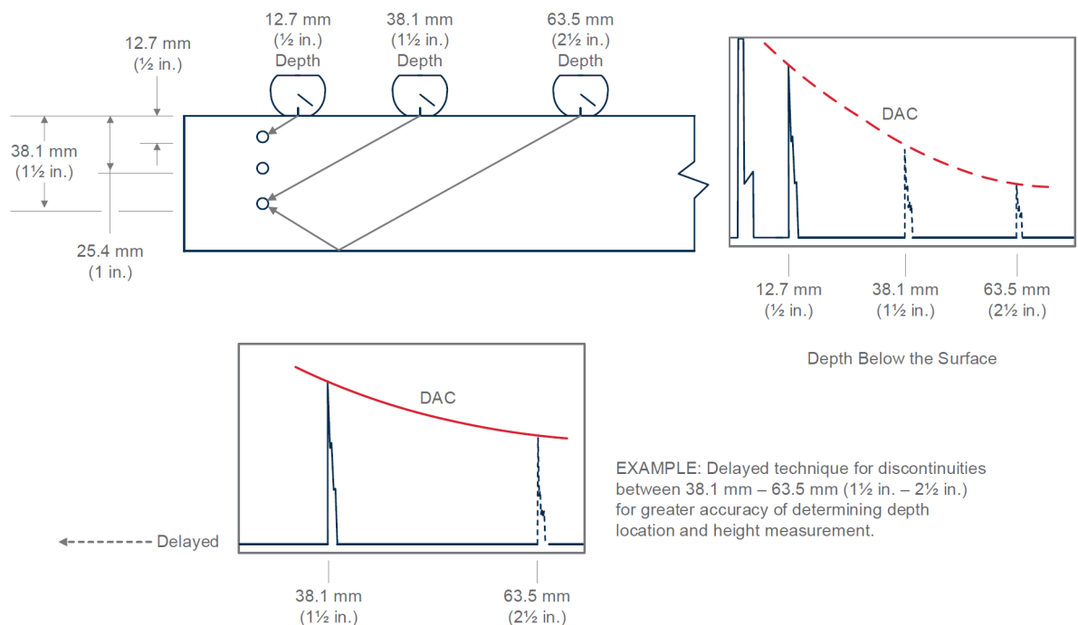
FIGURE 5 Shear Wave Distance and Sensitivity Calibration
