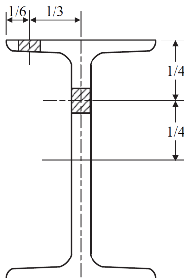
FIGURE 7 Position of the Test Samples – Flats and Rounds (Bars)
