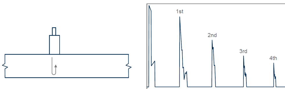
FIGURE 4 Compression Wave Sensitivity Calibration
