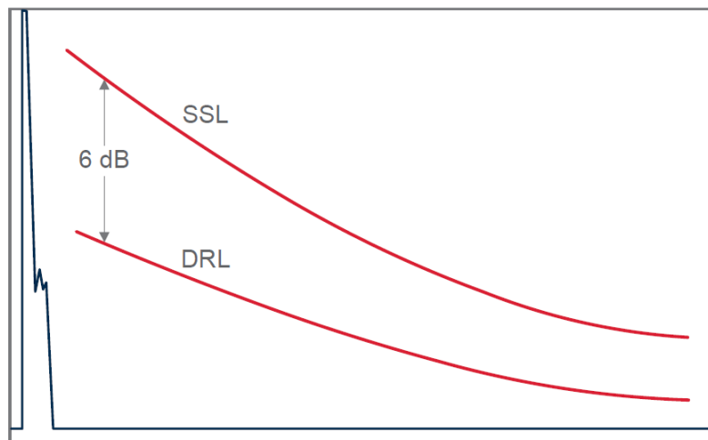
FIGURE 7 Screen Marking
