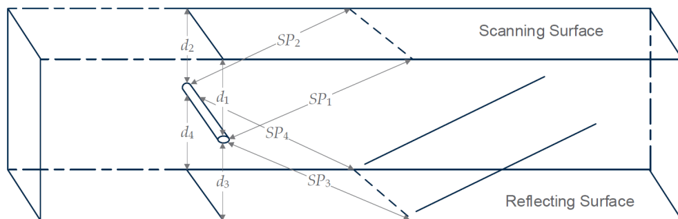
FIGURE 1 Standard Reference Reflector
