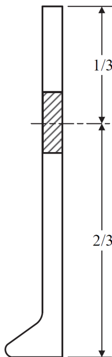
FIGURE 2 Position of the Test Samples – Bulb Flats
