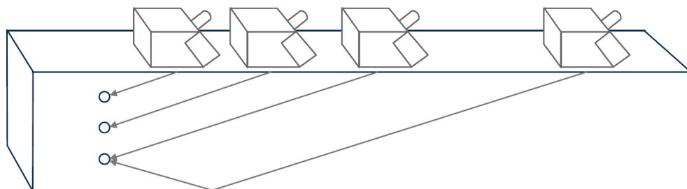
FIGURE 2 Recommended Calibration Block
