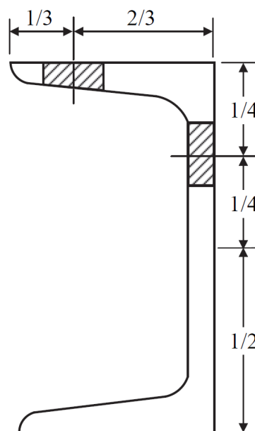
FIGURE 5 Position of the Test Samples – Channels and Beams
