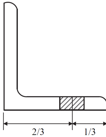
FIGURE 3 Position of the Test Samples – Angles
