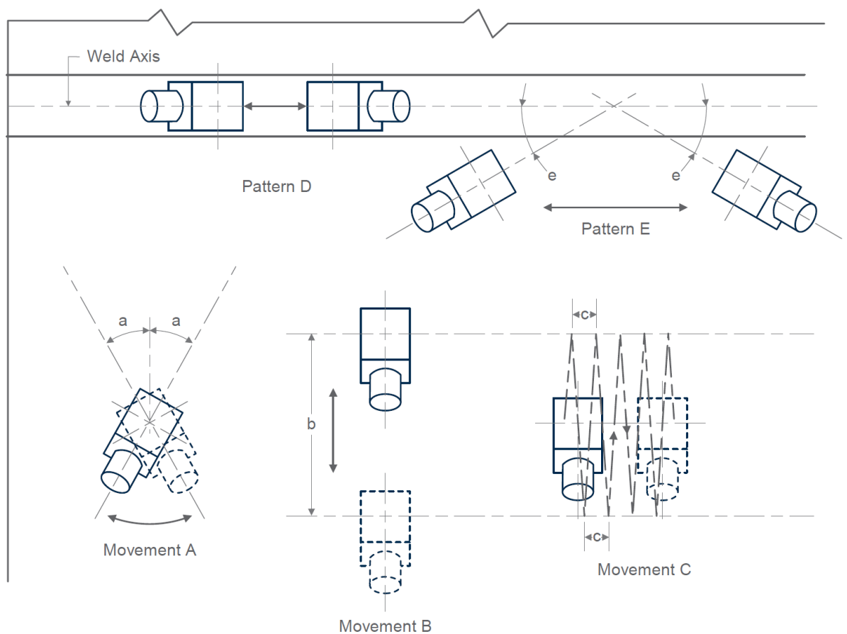
FIGURE 6 Plan View of UT Scanning Patterns
