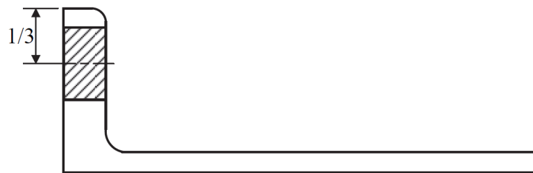
FIGURE 4 Position of the Test Samples – Unequal Angles
