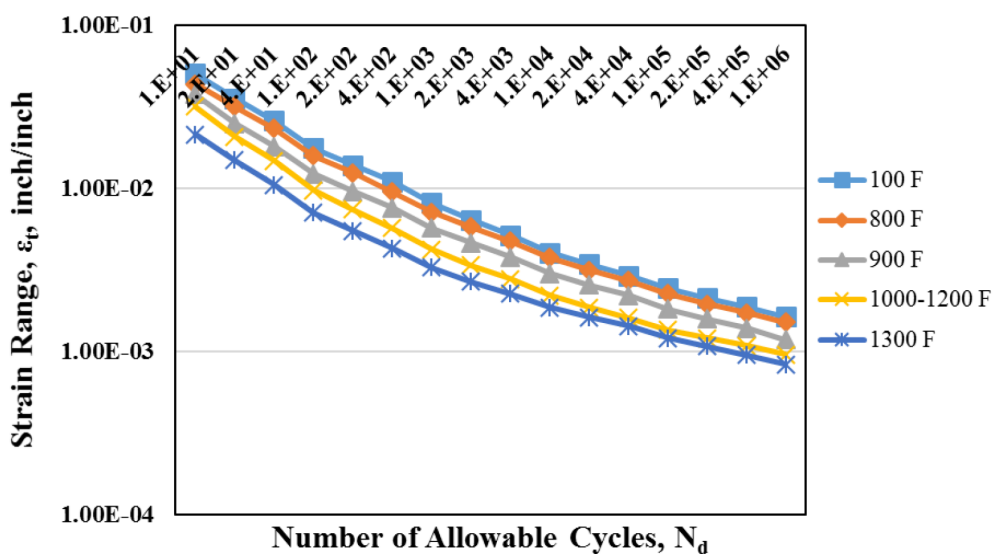
FIGURE 2 Design Fatigue Strain Range, \epsilon_p , for 316 Stainless Steel (1,2)
